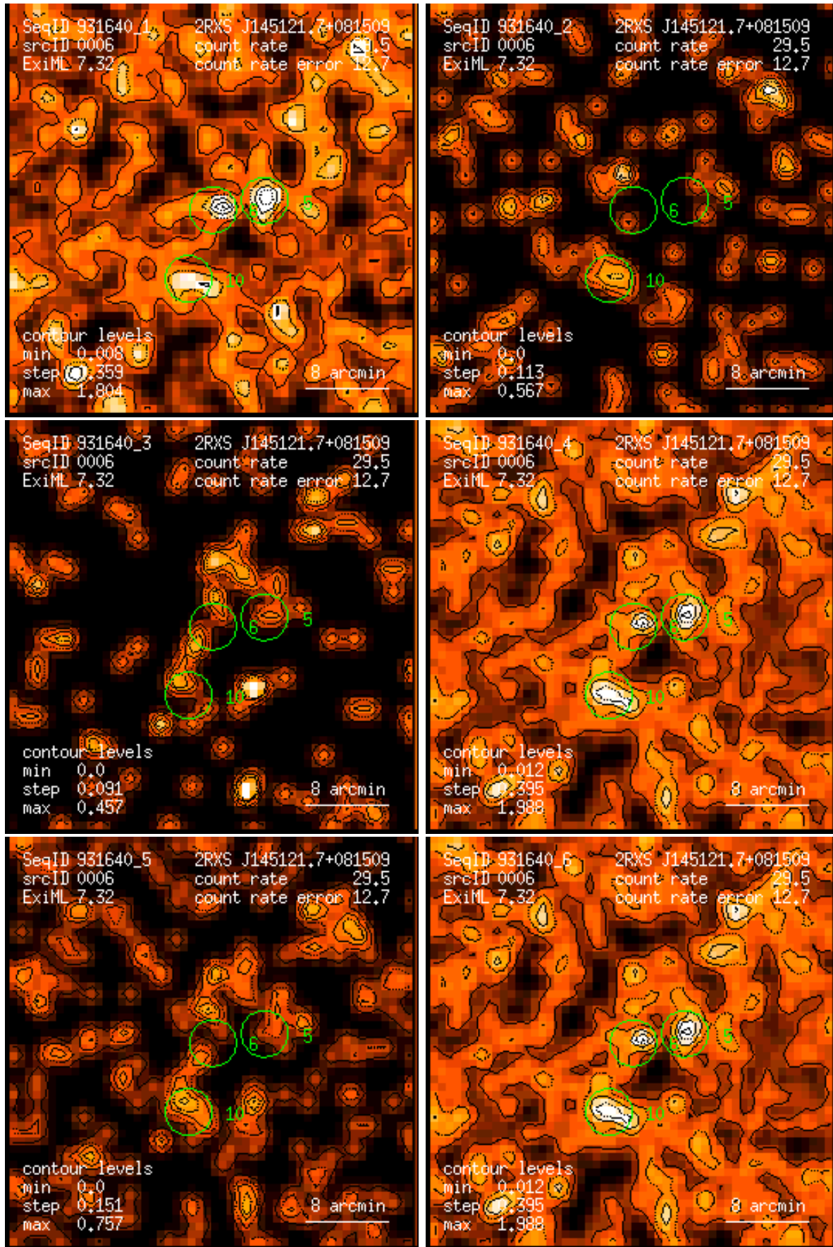
Figure 6: RASS 931640: detection 0006: band rate images, Gaussian filter: (1) PSPC channels 11 – 41, (2) 52 – 90, (3) 91 – 201, (4) 11 – 235, (5) 52 – 201, (6) 11 – 201. Broad band rates in counts/ks. Band rate contour levels in counts/ks/arcmin 2 .
