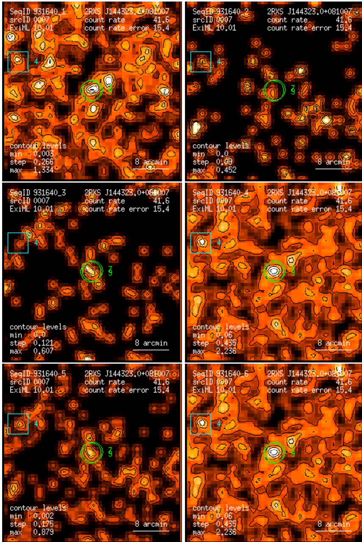
Figure 7: RASS 931640: detection 0007: band rate images, Gaussian filter: (1) PSPC channels 11 – 41, (2) 52 – 90, (3) 91 – 201, (4) 11 – 235, (5) 52 – 201, (6) 11 – 201. Broad band rates in counts/ks. Band rate contour levels in counts/ks/arcmin 2 .
