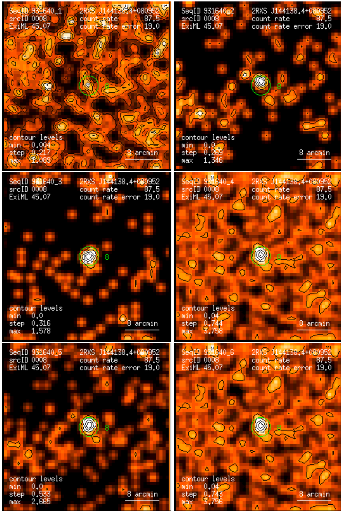
Figure 8: RASS 931640: detection 0008: band rate images, Gaussian filter: (1) PSPC channels 11 – 41, (2) 52 – 90, (3) 91 – 201, (4) 11 – 235, (5) 52 – 201, (6) 11 – 201. Broad band rates in counts/ks. Band rate contour levels in counts/ks/arcmin 2 .
