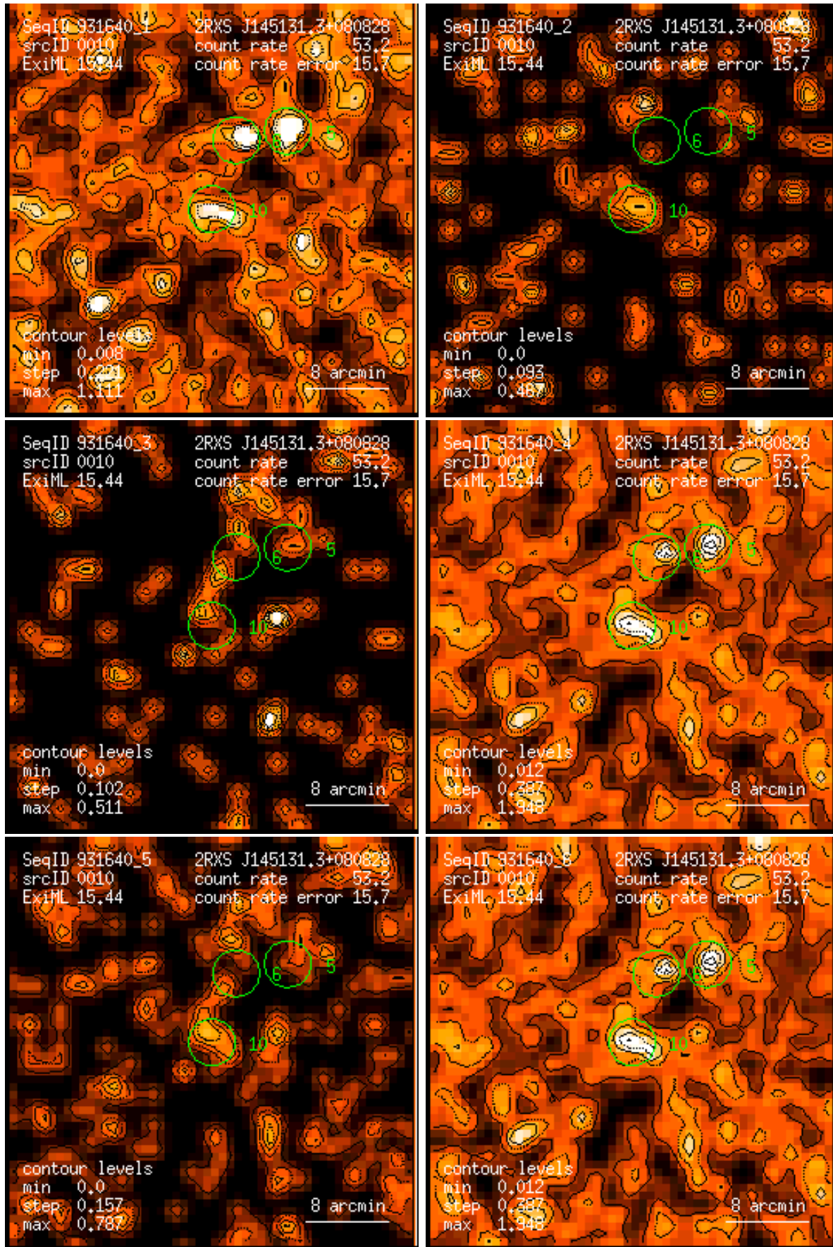
Figure 10: RASS 931640: detection 0010: band rate images, Gaussian filter: (1) PSPC channels 11 – 41, (2) 52 – 90, (3) 91 – 201, (4) 11 – 235, (5) 52 – 201, (6) 11 – 201. Broad band rates in counts/ks. Band rate contour levels in counts/ks/arcmin 2 .
