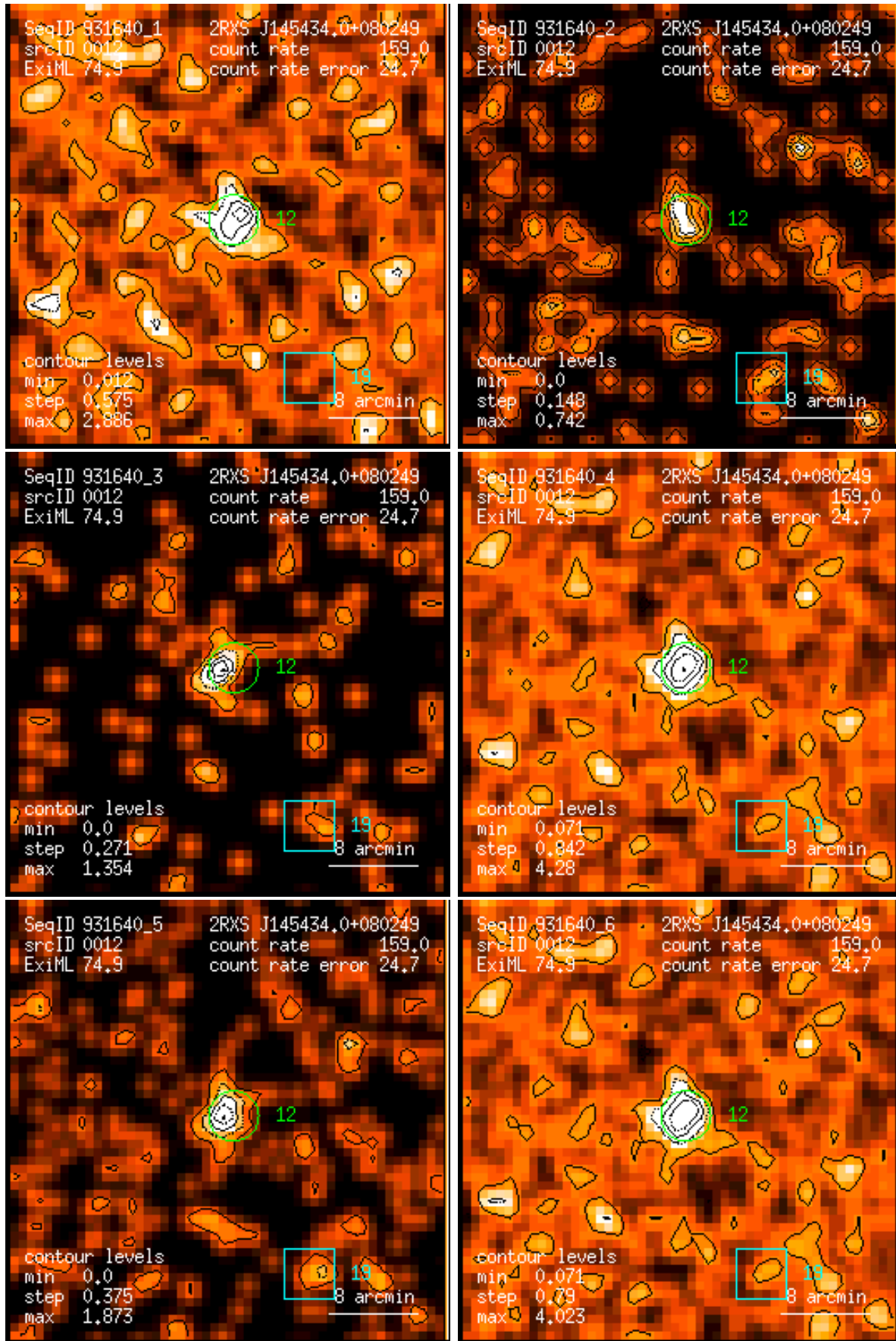
Figure 12: RASS 931640: detection 0012: band rate images, Gaussian filter: (1) PSPC channels 11 – 41, (2) 52 – 90, (3) 91 – 201, (4) 11 – 235, (5) 52 – 201, (6) 11 – 201. Broad band rates in counts/ks. Band rate contour levels in counts/ks/arcmin 2 .
