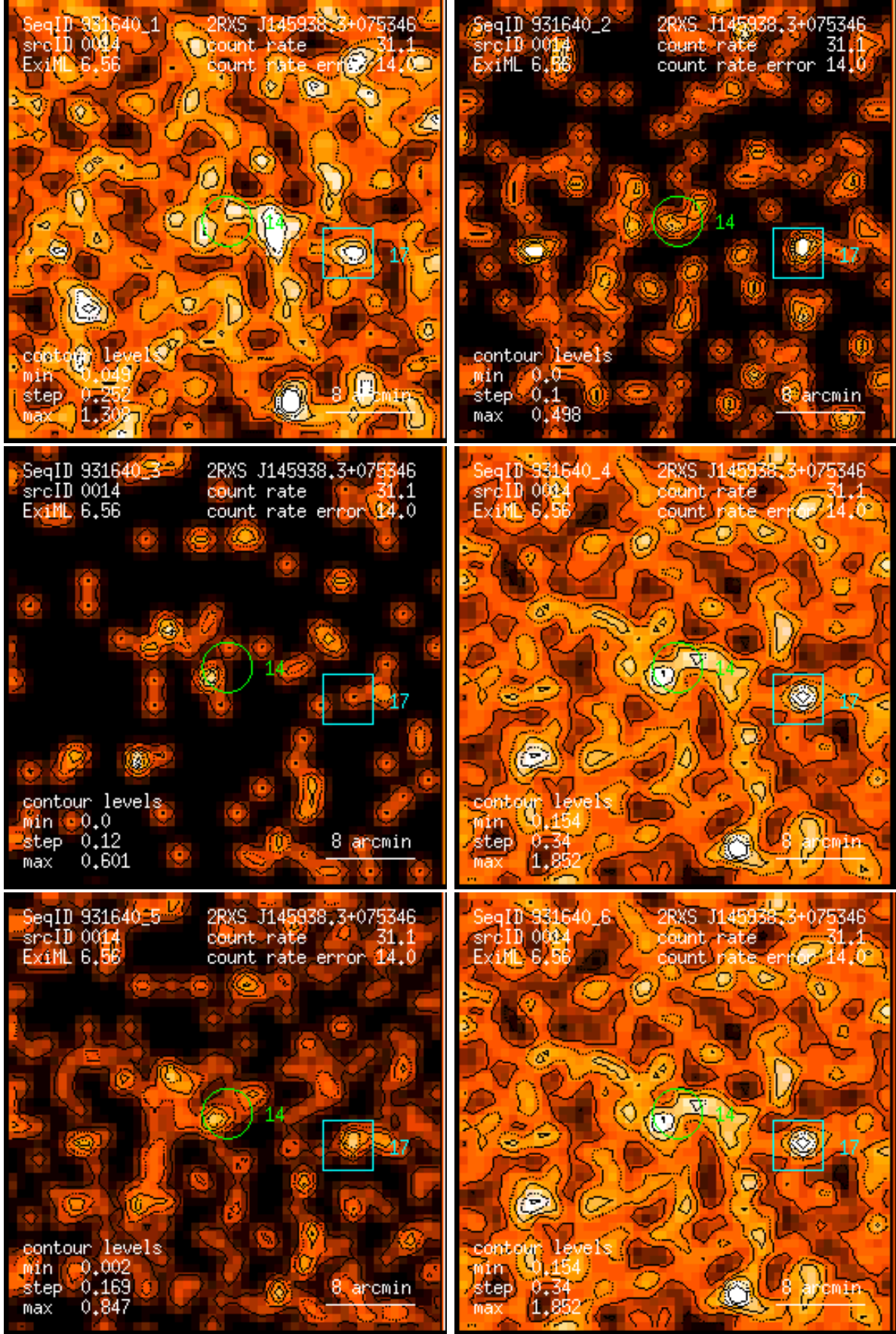
Figure 14: RASS 931640: detection 0014: band rate images, Gaussian filter: (1) PSPC channels 11 – 41, (2) 52 – 90, (3) 91 – 201, (4) 11 – 235, (5) 52 – 201, (6) 11 – 201. Broad band rates in counts/ks. Band rate contour levels in counts/ks/arcmin 2 .
