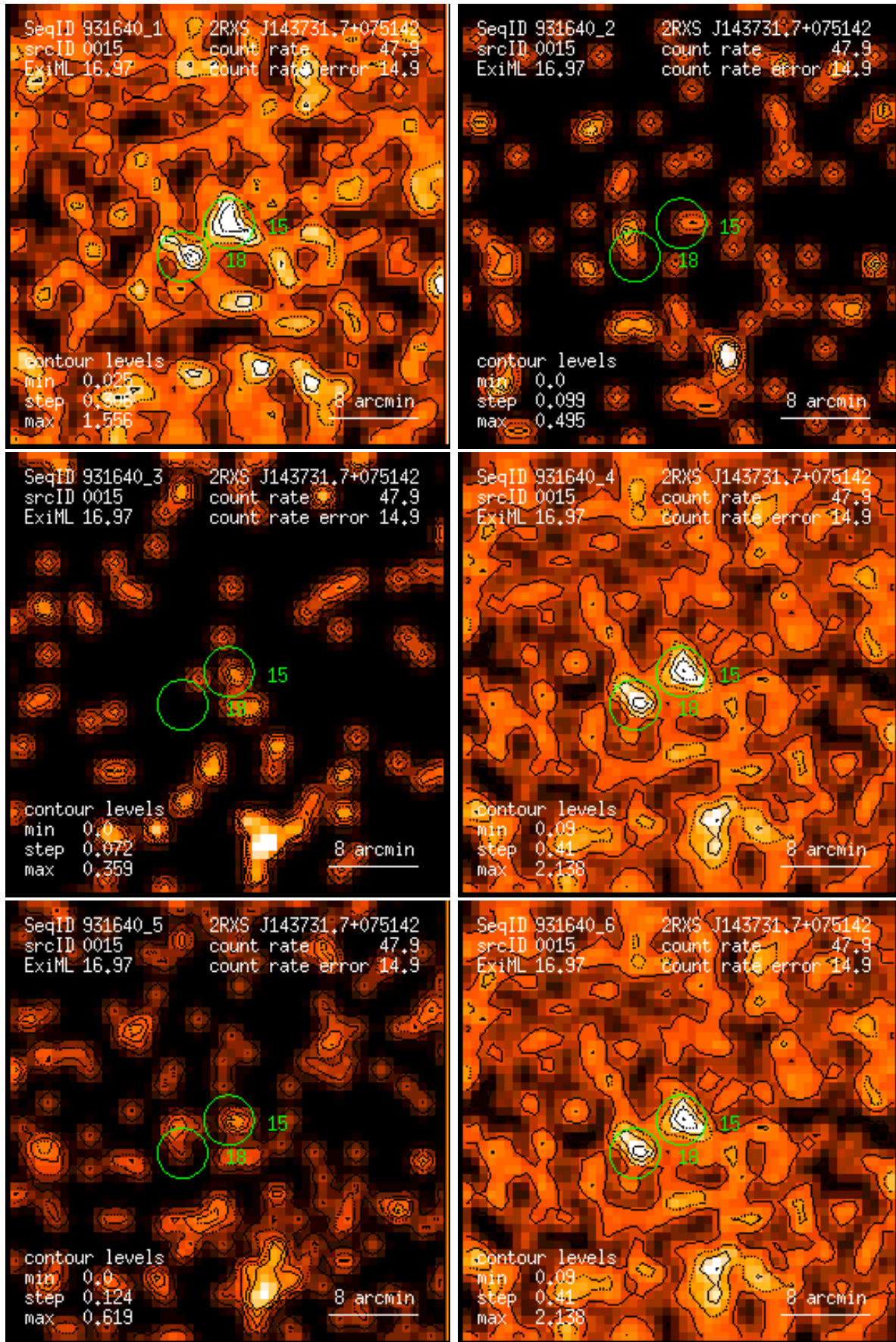
Figure 15: RASS 931640: detection 0015: band rate images, Gaussian filter: (1) PSPC channels 11 – 41, (2) 52 – 90, (3) 91 – 201, (4) 11 – 235, (5) 52 – 201, (6) 11 – 201. Broad band rates in counts/ks. Band rate contour levels in counts/ks/arcmin 2 .
