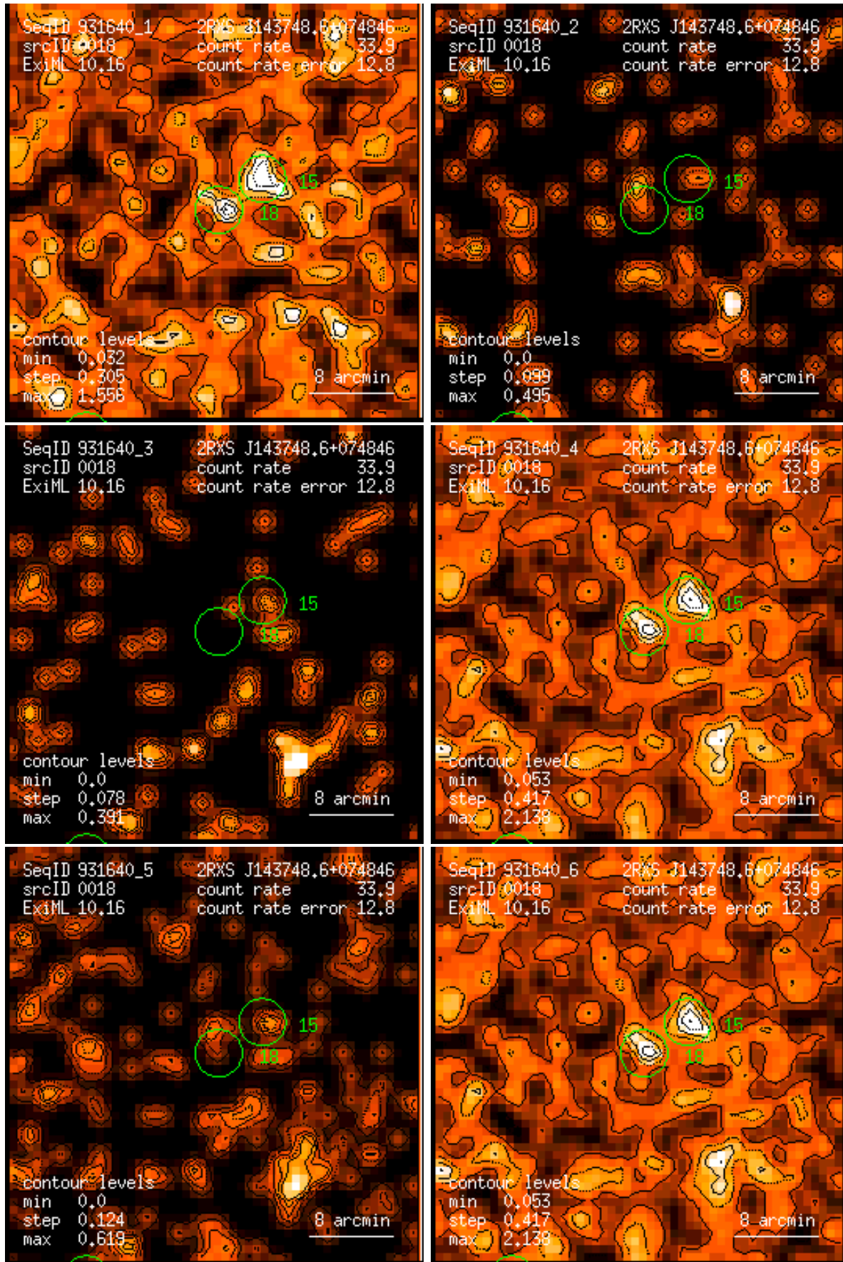
Figure 18: RASS 931640: detection 0018: band rate images, Gaussian filter: (1) PSPC channels 11 – 41, (2) 52 – 90, (3) 91 – 201, (4) 11 – 235, (5) 52 – 201, (6) 11 – 201. Broad band rates in counts/ks. Band rate contour levels in counts/ks/arcmin 2 .
