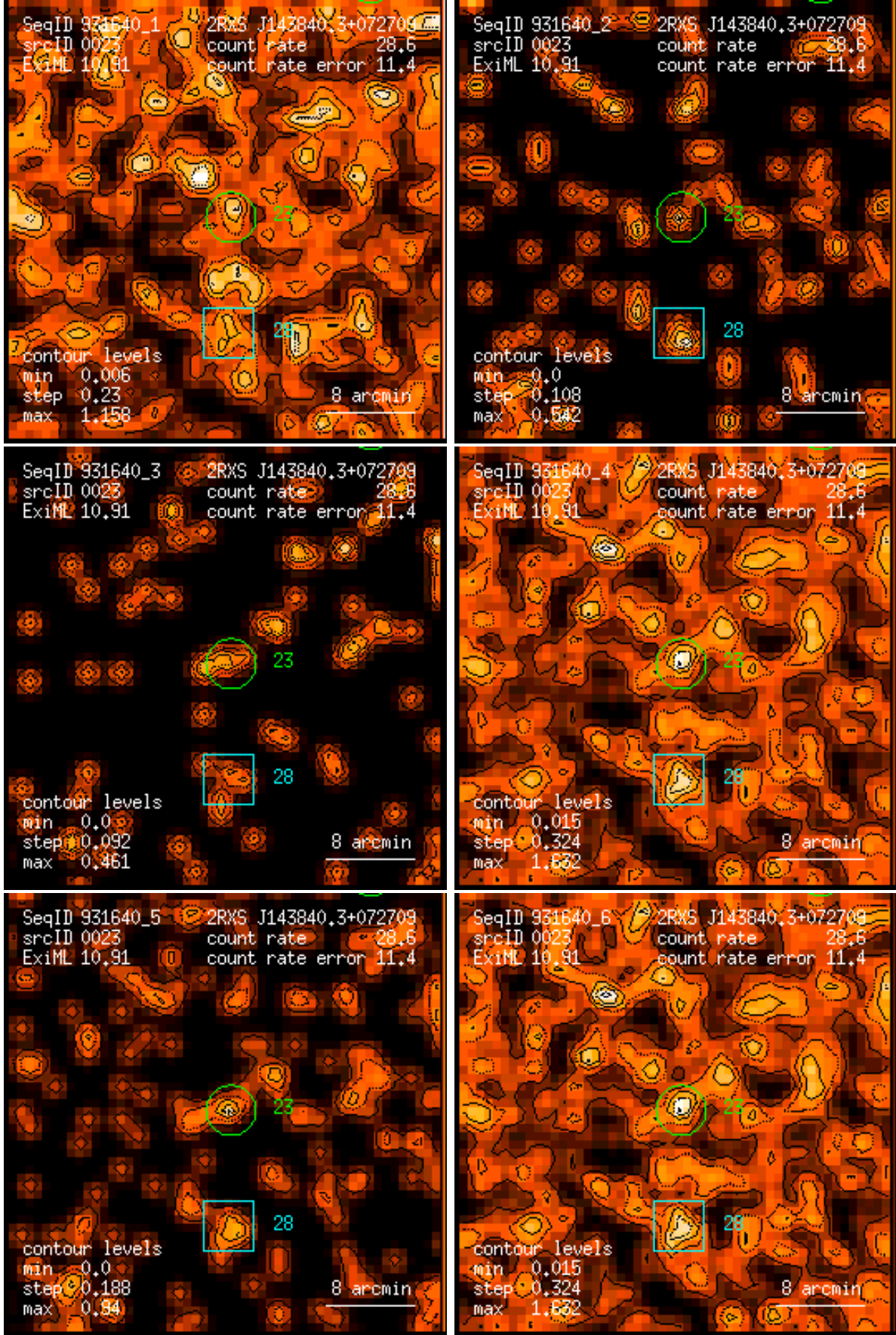
Figure 23: RASS 931640: detection 0023: band rate images, Gaussian filter: (1) PSPC channels 11 – 41, (2) 52 – 90, (3) 91 – 201, (4) 11 – 235, (5) 52 – 201, (6) 11 – 201. Broad band rates in counts/ks. Band rate contour levels in counts/ks/arcmin 2 .
