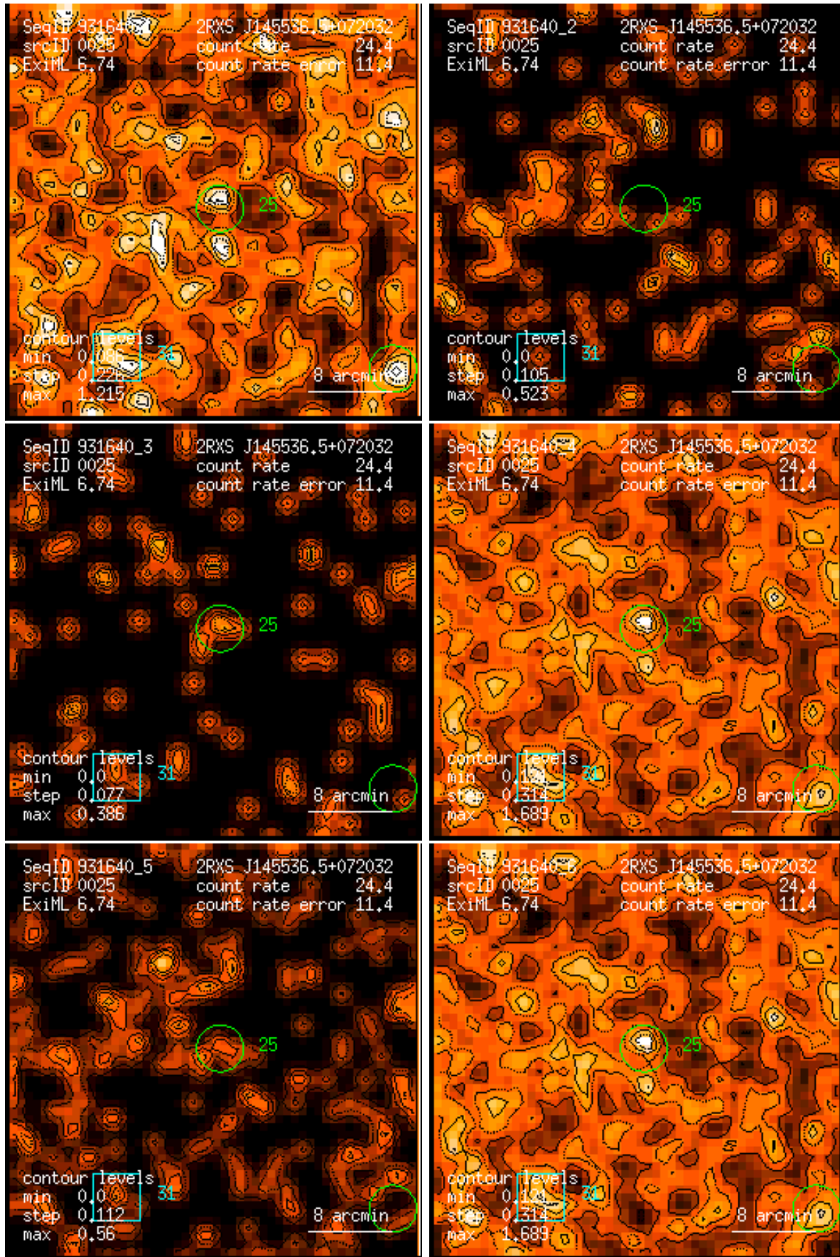
Figure 25: RASS 931640: detection 0025: band rate images, Gaussian filter: (1) PSPC channels 11 – 41, (2) 52 – 90, (3) 91 – 201, (4) 11 – 235, (5) 52 – 201, (6) 11 – 201. Broad band rates in counts/ks. Band rate contour levels in counts/ks/arcmin 2 .
