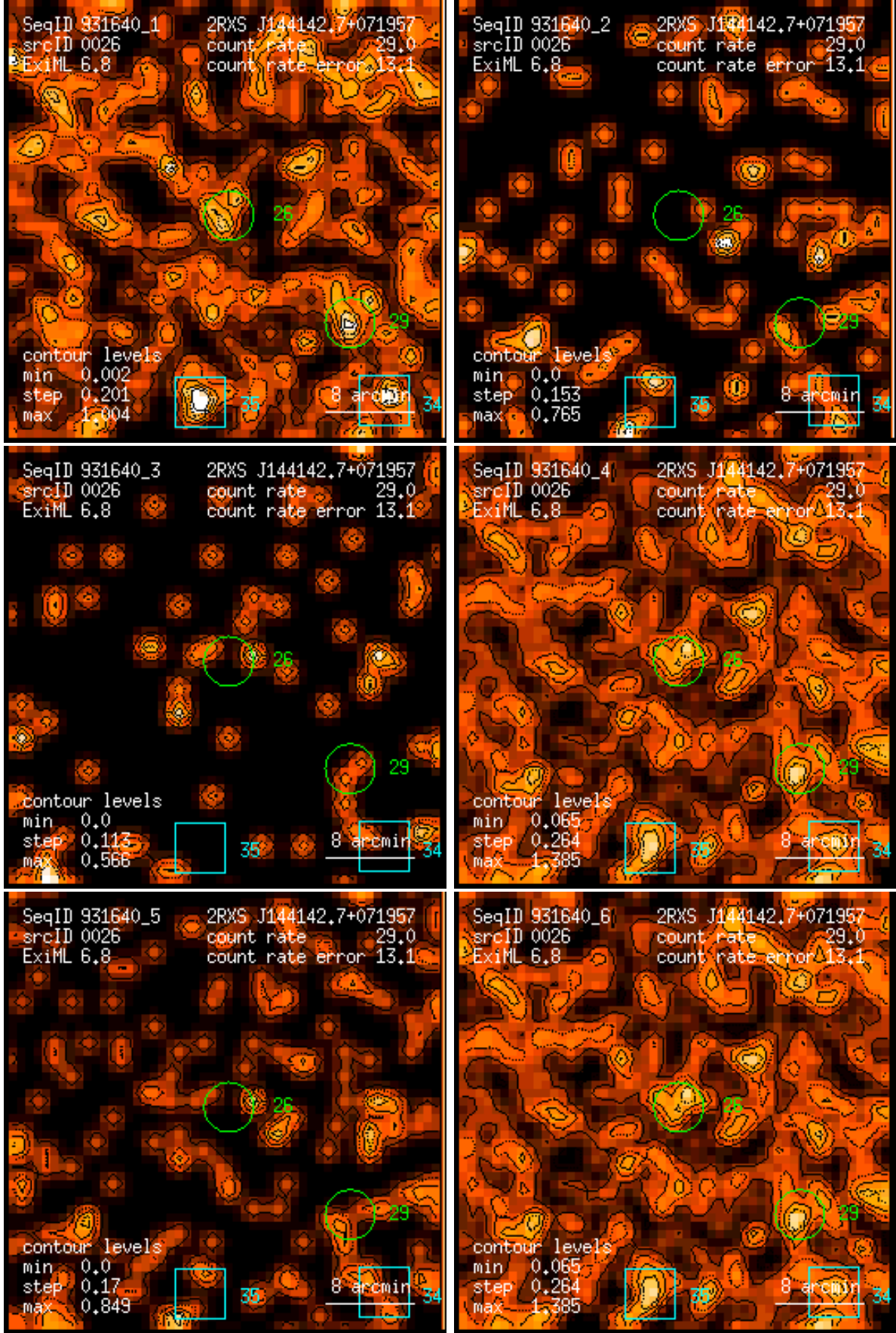
Figure 26: RASS 931640: detection 0026: band rate images, Gaussian filter: (1) PSPC channels 11 – 41, (2) 52 – 90, (3) 91 – 201, (4) 11 – 235, (5) 52 – 201, (6) 11 – 201. Broad band rates in counts/ks. Band rate contour levels in counts/ks/arcmin 2 .
