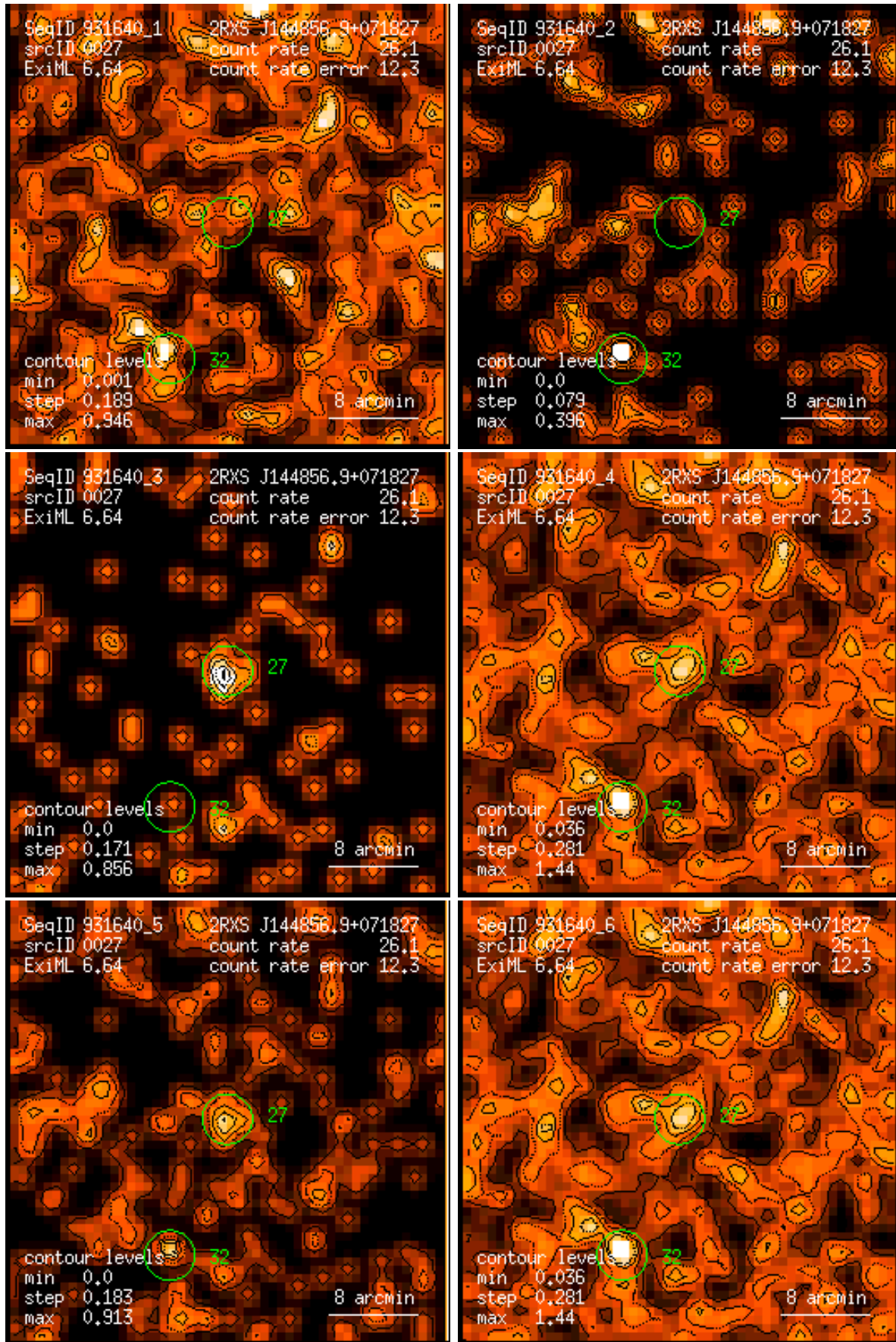
Figure 27: RASS 931640: detection 0027: band rate images, Gaussian filter: (1) PSPC channels 11 – 41, (2) 52 – 90, (3) 91 – 201, (4) 11 – 235, (5) 52 – 201, (6) 11 – 201. Broad band rates in counts/ks. Band rate contour levels in counts/ks/arcmin 2 .
