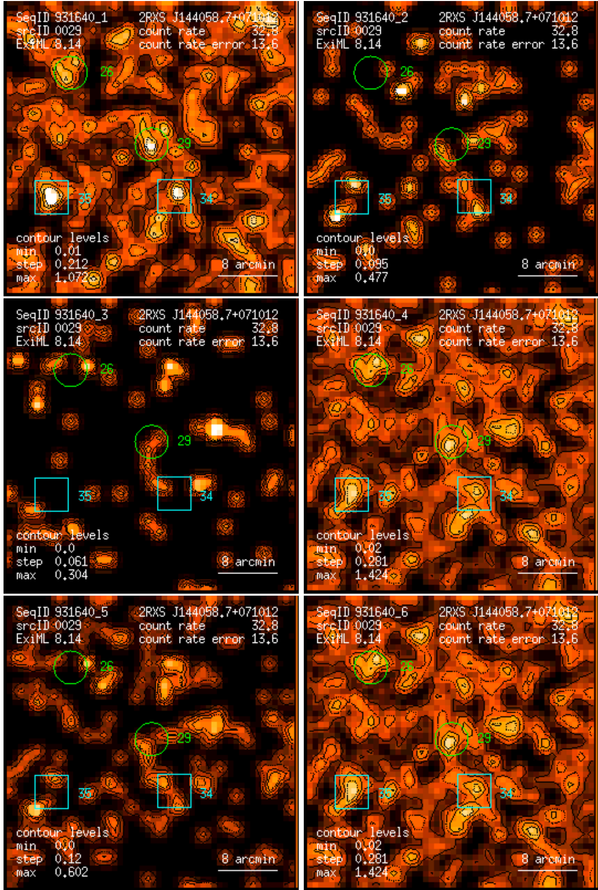
Figure 29: RASS 931640: detection 0029: band rate images, Gaussian filter: (1) PSPC channels 11 – 41, (2) 52 – 90, (3) 91 – 201, (4) 11 – 235, (5) 52 – 201, (6) 11 – 201. Broad band rates in counts/ks. Band rate contour levels in counts/ks/arcmin 2 .
