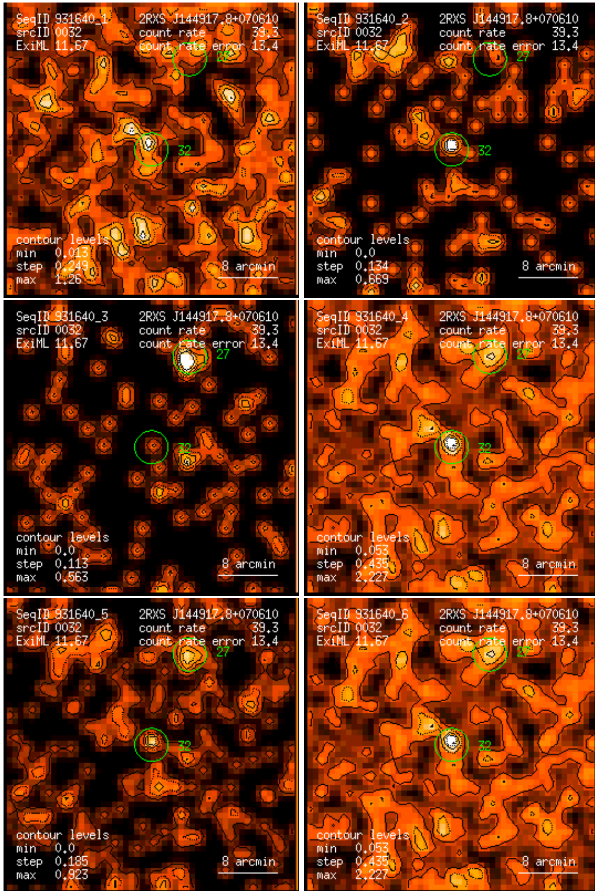
Figure 32: RASS 931640: detection 0032: band rate images, Gaussian filter: (1) PSPC channels 11 – 41, (2) 52 – 90, (3) 91 – 201, (4) 11 – 235, (5) 52 – 201, (6) 11 – 201. Broad band rates in counts/ks. Band rate contour levels in counts/ks/arcmin 2 .
