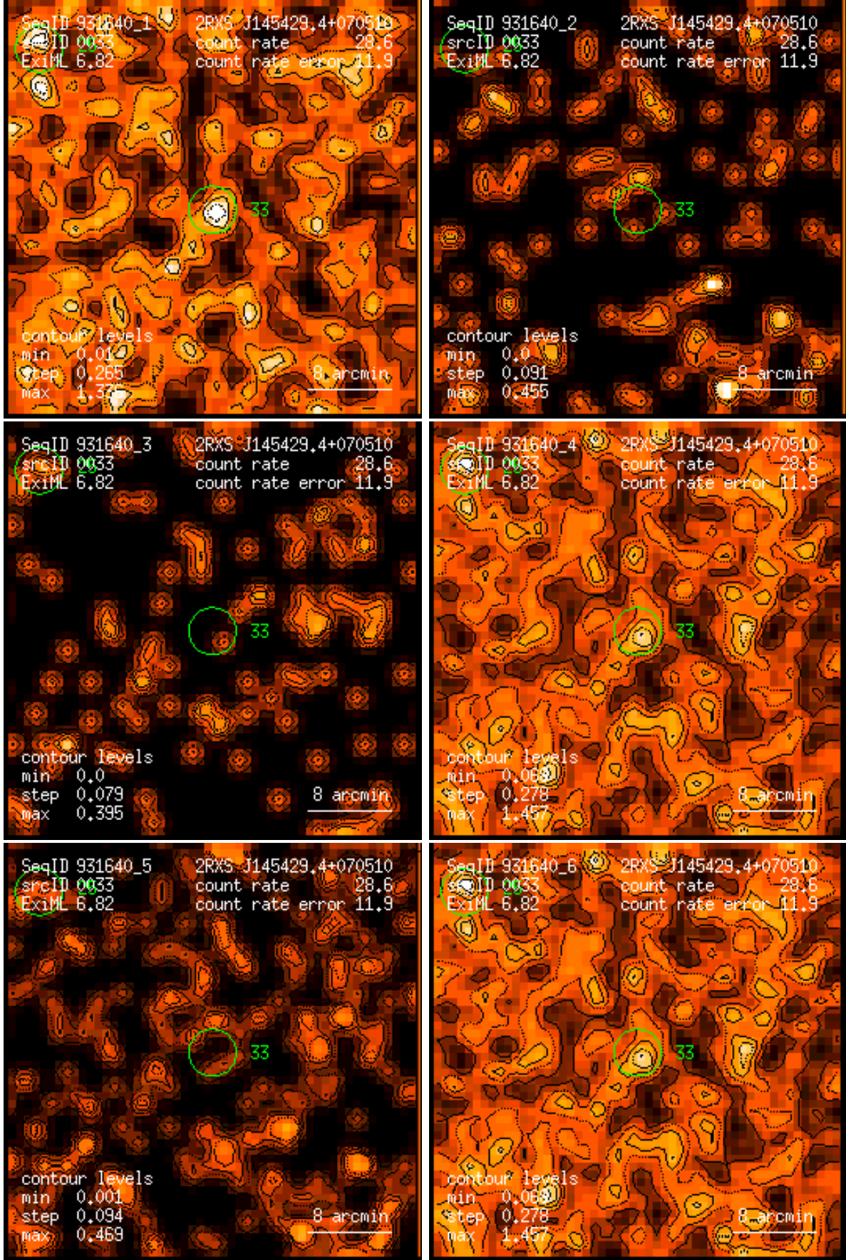
Figure 33: RASS 931640: detection 0033: band rate images, Gaussian filter: (1) PSPC channels 11 – 41, (2) 52 – 90, (3) 91 – 201, (4) 11 – 235, (5) 52 – 201, (6) 11 – 201. Broad band rates in counts/ks. Band rate contour levels in counts/ks/arcmin 2 .
