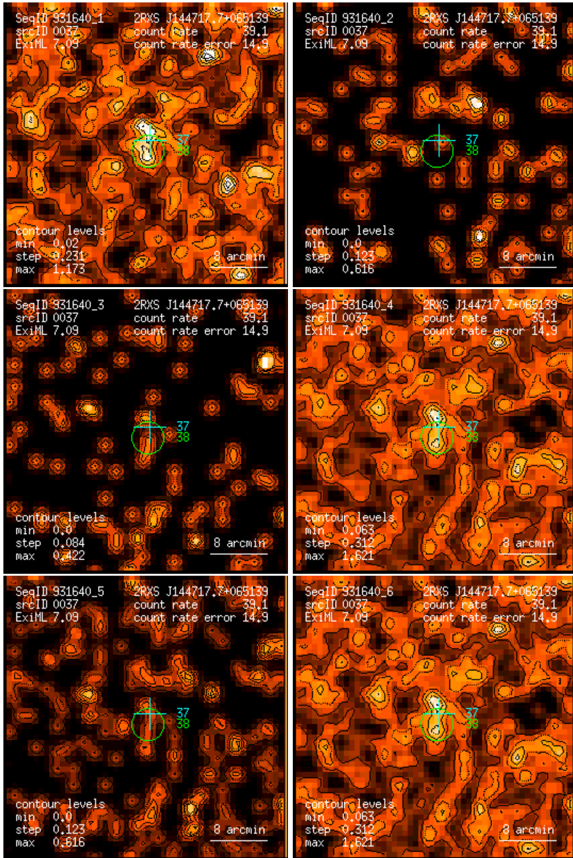
Figure 37: RASS 931640: detection 0037: band rate images, Gaussian filter: (1) PSPC channels 11 – 41, (2) 52 – 90, (3) 91 – 201, (4) 11 – 235, (5) 52 – 201, (6) 11 – 201. Broad band rates in counts/ks. Band rate contour levels in counts/ks/arcmin 2 .
