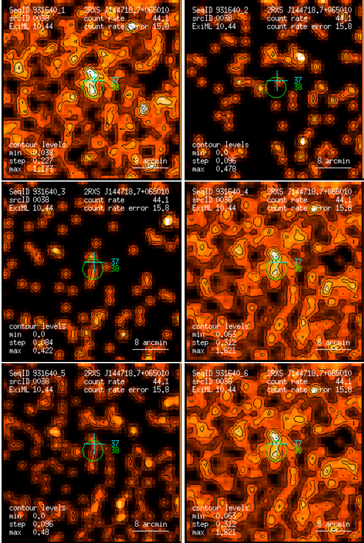
Figure 38: RASS 931640: detection 0038: band rate images, Gaussian filter: (1) PSPC channels 11 – 41, (2) 52 – 90, (3) 91 – 201, (4) 11 – 235, (5) 52 – 201, (6) 11 – 201. Broad band rates in counts/ks. Band rate contour levels in counts/ks/arcmin 2 .
