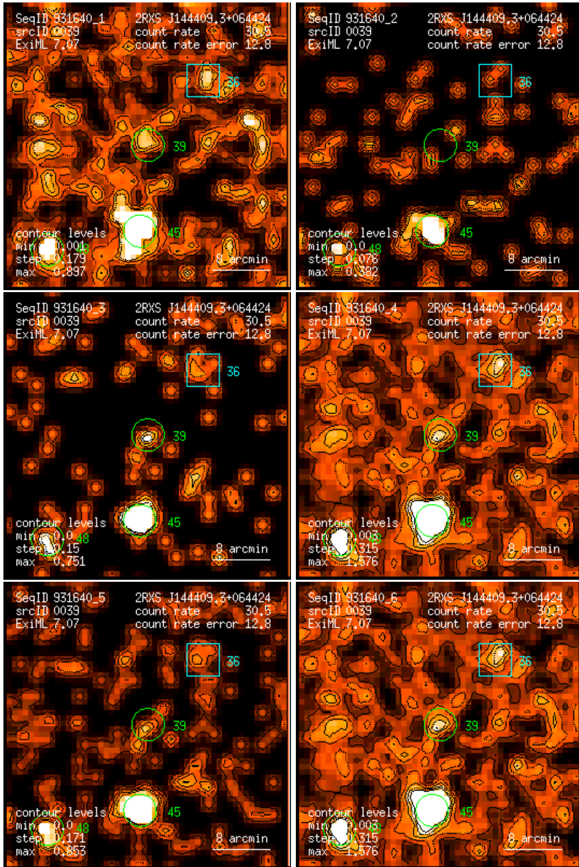
Figure 39: RASS 931640: detection 0039: band rate images, Gaussian filter: (1) PSPC channels 11 – 41, (2) 52 – 90, (3) 91 – 201, (4) 11 – 235, (5) 52 – 201, (6) 11 – 201. Broad band rates in counts/ks. Band rate contour levels in counts/ks/arcmin 2 .
