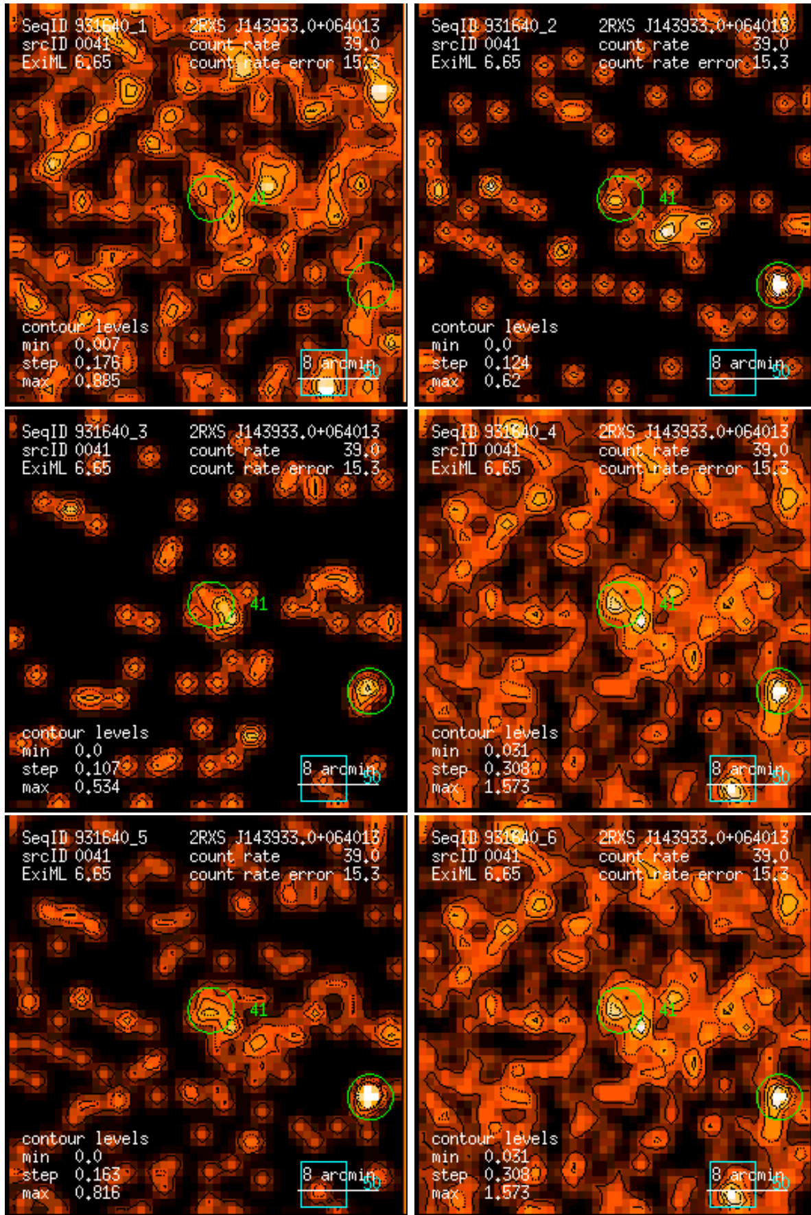
Figure 41: RASS 931640: detection 0041: band rate images, Gaussian filter: (1) PSPC channels 11 – 41, (2) 52 – 90, (3) 91 – 201, (4) 11 – 235, (5) 52 – 201, (6) 11 – 201. Broad band rates in counts/ks. Band rate contour levels in counts/ks/arcmin 2 .
