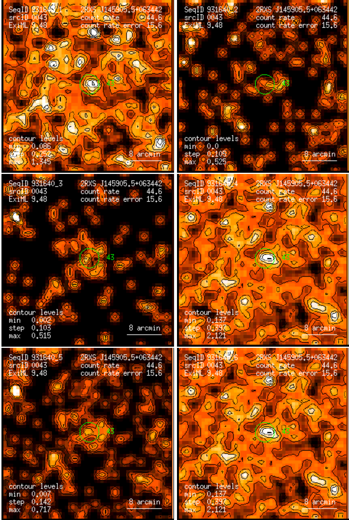
Figure 43: RASS 931640: detection 0043: band rate images, Gaussian filter: (1) PSPC channels 11 – 41, (2) 52 – 90, (3) 91 – 201, (4) 11 – 235, (5) 52 – 201, (6) 11 – 201. Broad band rates in counts/ks. Band rate contour levels in counts/ks/arcmin 2 .
