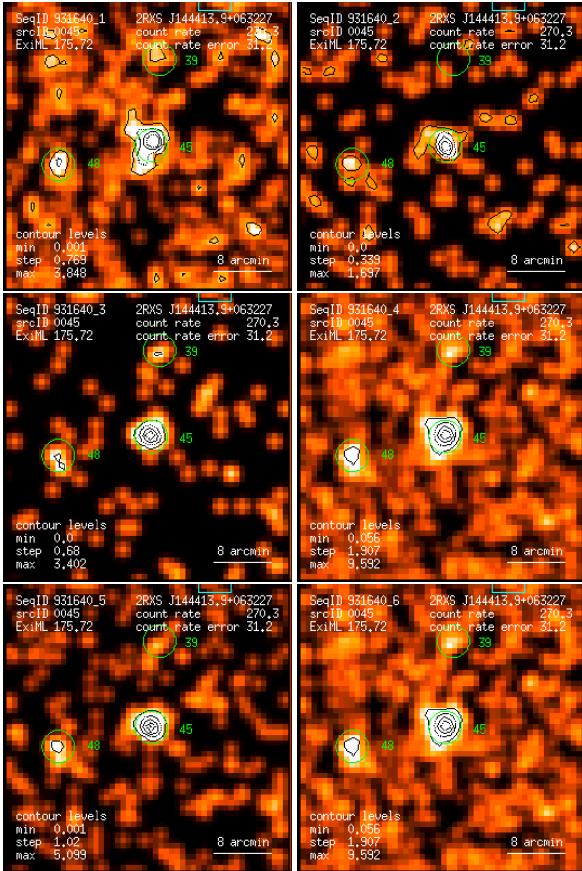
Figure 45: RASS 931640: detection 0045: band rate images, Gaussian filter: (1) PSPC channels 11 – 41, (2) 52 – 90, (3) 91 – 201, (4) 11 – 235, (5) 52 – 201, (6) 11 – 201. Broad band rates in counts/ks. Band rate contour levels in counts/ks/arcmin 2 .
