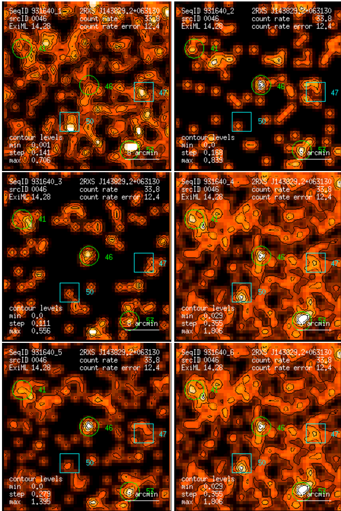
Figure 46: RASS 931640: detection 0046: band rate images, Gaussian filter: (1) PSPC channels 11 – 41, (2) 52 – 90, (3) 91 – 201, (4) 11 – 235, (5) 52 – 201, (6) 11 – 201. Broad band rates in counts/ks. Band rate contour levels in counts/ks/arcmin 2 .
