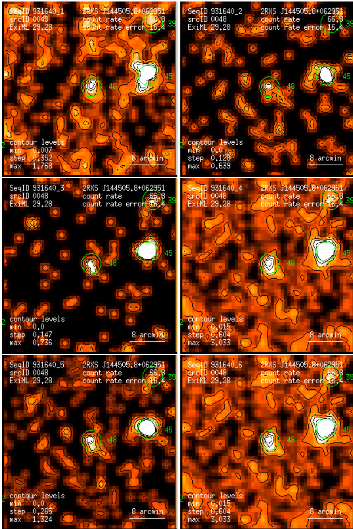
Figure 48: RASS 931640: detection 0048: band rate images, Gaussian filter: (1) PSPC channels 11 – 41, (2) 52 – 90, (3) 91 – 201, (4) 11 – 235, (5) 52 – 201, (6) 11 – 201. Broad band rates in counts/ks. Band rate contour levels in counts/ks/arcmin 2 .
