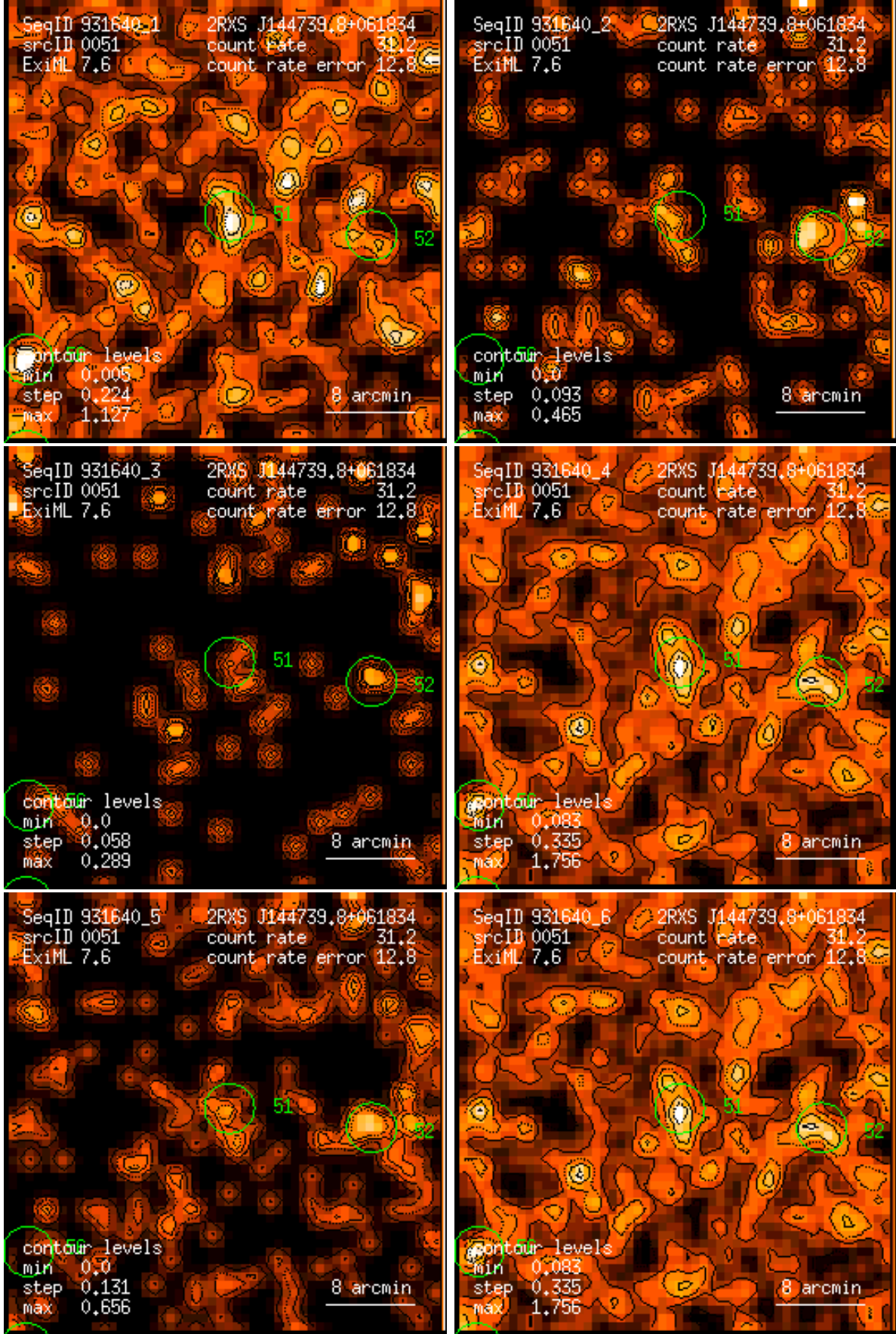
Figure 51: RASS 931640: detection 0051: band rate images, Gaussian filter: (1) PSPC channels 11 – 41, (2) 52 – 90, (3) 91 – 201, (4) 11 – 235, (5) 52 – 201, (6) 11 – 201. Broad band rates in counts/ks. Band rate contour levels in counts/ks/arcmin 2 .
