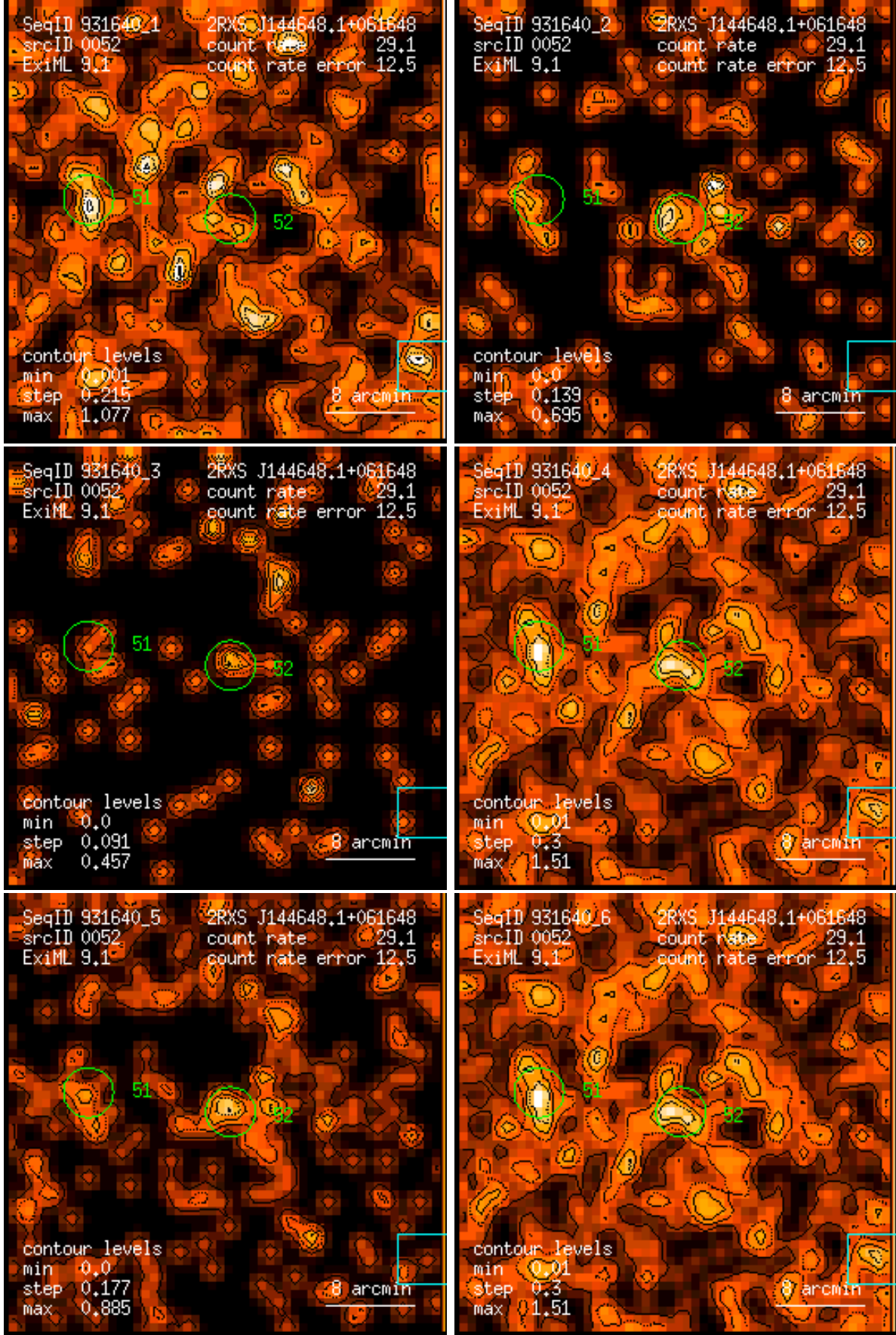
Figure 52: RASS 931640: detection 0052: band rate images, Gaussian filter: (1) PSPC channels 11 – 41, (2) 52 – 90, (3) 91 – 201, (4) 11 – 235, (5) 52 – 201, (6) 11 – 201. Broad band rates in counts/ks. Band rate contour levels in counts/ks/arcmin 2 .
