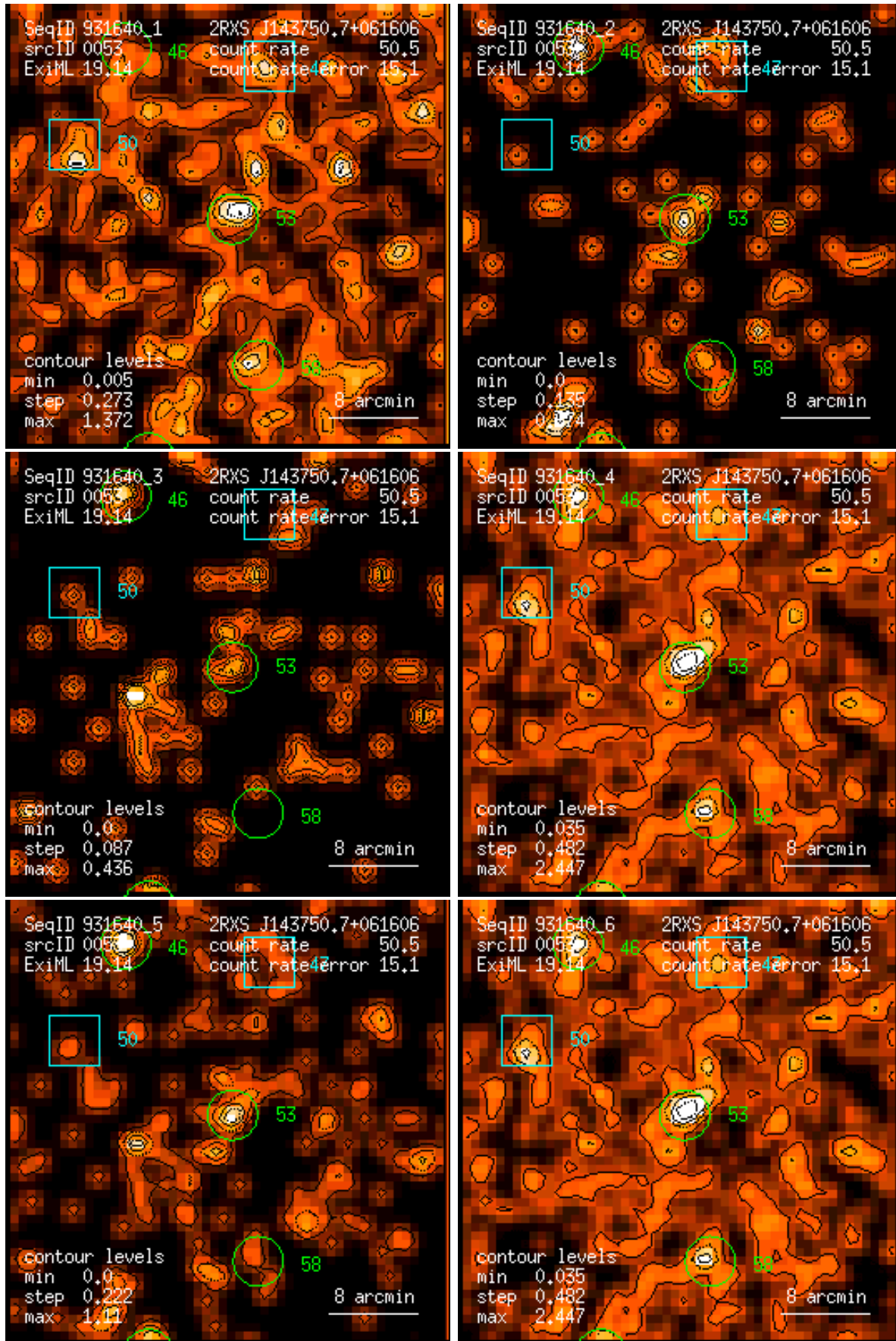
Figure 53: RASS 931640: detection 0053: band rate images, Gaussian filter: (1) PSPC channels 11 – 41, (2) 52 – 90, (3) 91 – 201, (4) 11 – 235, (5) 52 – 201, (6) 11 – 201. Broad band rates in counts/ks. Band rate contour levels in counts/ks/arcmin 2 .
