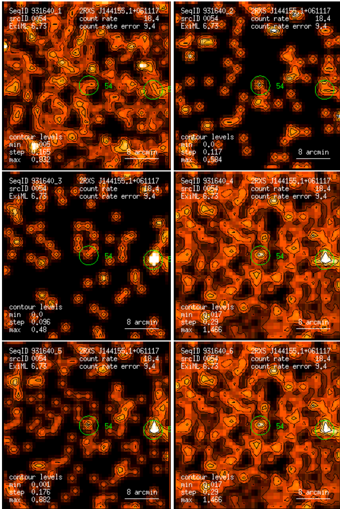
Figure 54: RASS 931640: detection 0054: band rate images, Gaussian filter: (1) PSPC channels 11 – 41, (2) 52 – 90, (3) 91 – 201, (4) 11 – 235, (5) 52 – 201, (6) 11 – 201. Broad band rates in counts/ks. Band rate contour levels in counts/ks/arcmin 2 .
