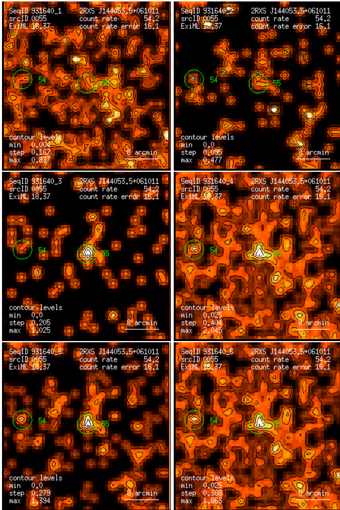
Figure 55: RASS 931640: detection 0055: band rate images, Gaussian filter: (1) PSPC channels 11 – 41, (2) 52 – 90, (3) 91 – 201, (4) 11 – 235, (5) 52 – 201, (6) 11 – 201. Broad band rates in counts/ks. Band rate contour levels in counts/ks/arcmin 2 .
