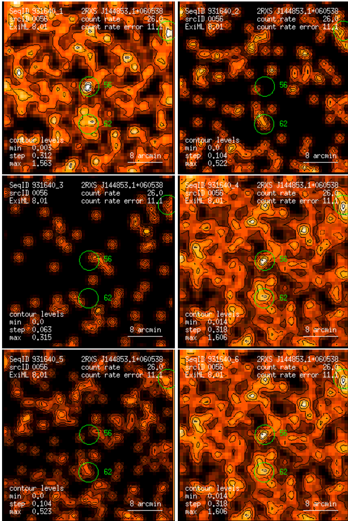
Figure 56: RASS 931640: detection 0056: band rate images, Gaussian filter: (1) PSPC channels 11 – 41, (2) 52 – 90, (3) 91 – 201, (4) 11 – 235, (5) 52 – 201, (6) 11 – 201. Broad band rates in counts/ks. Band rate contour levels in counts/ks/arcmin 2 .
