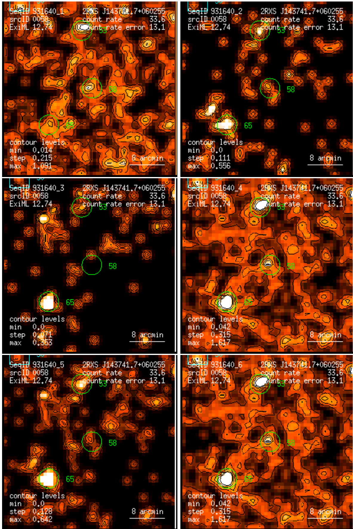
Figure 58: RASS 931640: detection 0058: band rate images, Gaussian filter: (1) PSPC channels 11 – 41, (2) 52 – 90, (3) 91 – 201, (4) 11 – 235, (5) 52 – 201, (6) 11 – 201. Broad band rates in counts/ks. Band rate contour levels in counts/ks/arcmin 2 .
