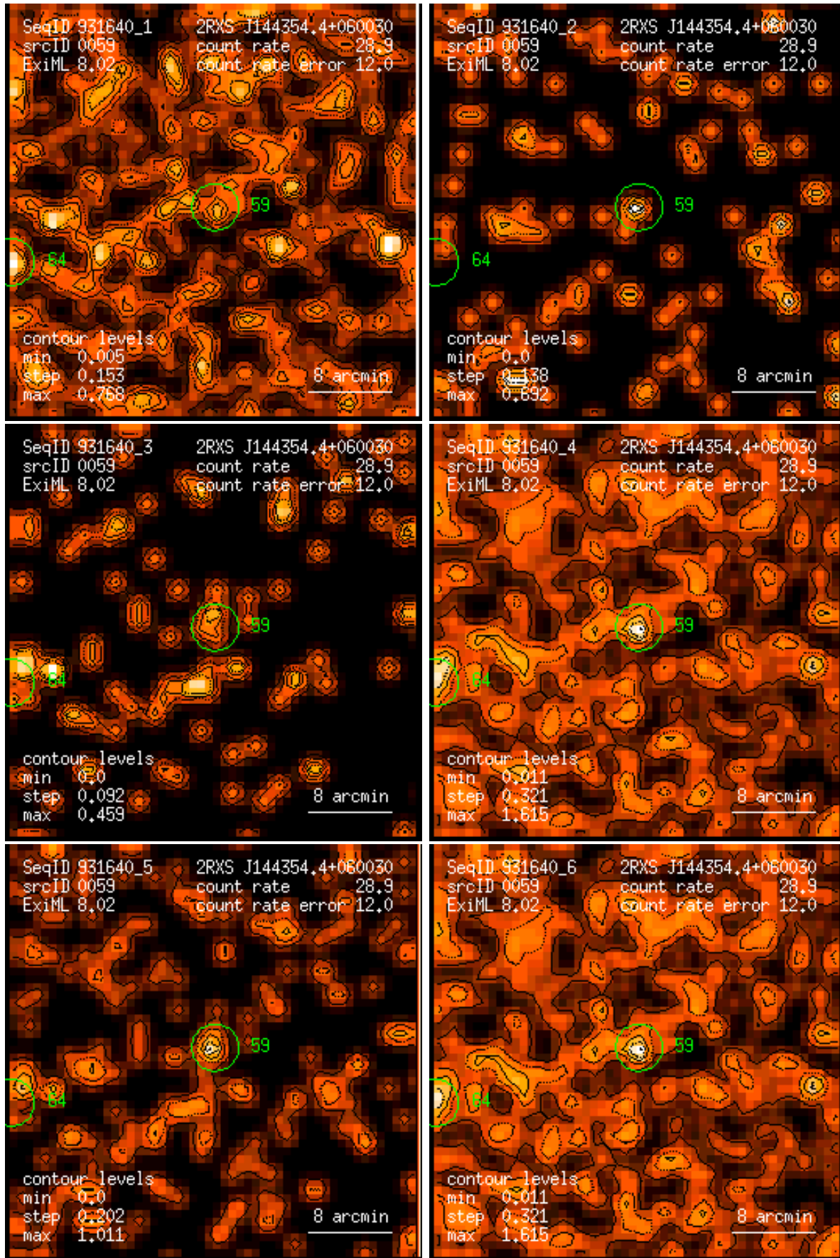
Figure 59: RASS 931640: detection 0059: band rate images, Gaussian filter: (1) PSPC channels 11 – 41, (2) 52 – 90, (3) 91 – 201, (4) 11 – 235, (5) 52 – 201, (6) 11 – 201. Broad band rates in counts/ks. Band rate contour levels in counts/ks/arcmin 2 .
