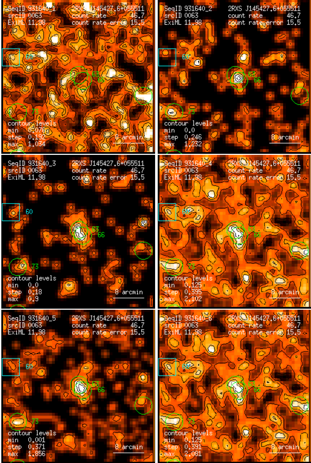
Figure 63: RASS 931640: detection 0063: band rate images, Gaussian filter: (1) PSPC channels 11 – 41, (2) 52 – 90, (3) 91 – 201, (4) 11 – 235, (5) 52 – 201, (6) 11 – 201. Broad band rates in counts/ks. Band rate contour levels in counts/ks/arcmin 2 .
