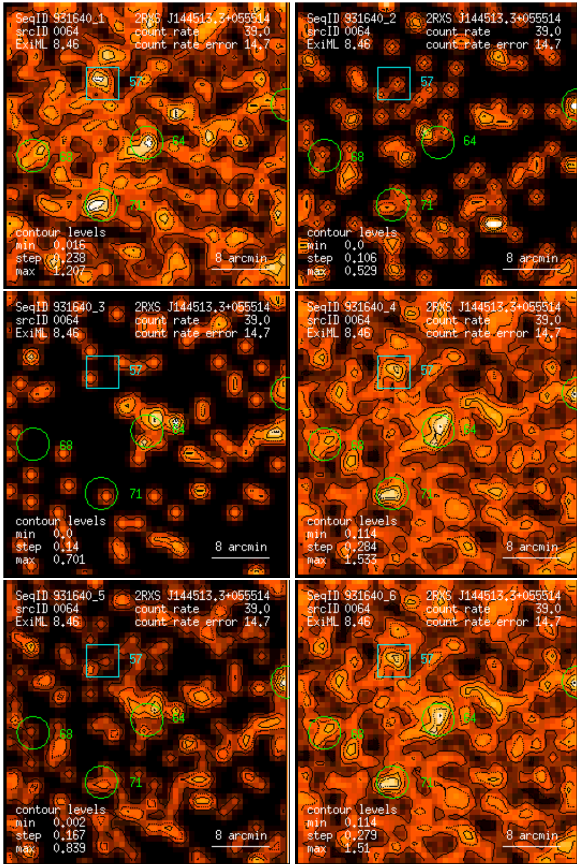
Figure 64: RASS 931640: detection 0064: band rate images, Gaussian filter: (1) PSPC channels 11 – 41, (2) 52 – 90, (3) 91 – 201, (4) 11 – 235, (5) 52 – 201, (6) 11 – 201. Broad band rates in counts/ks. Band rate contour levels in counts/ks/arcmin 2 .
