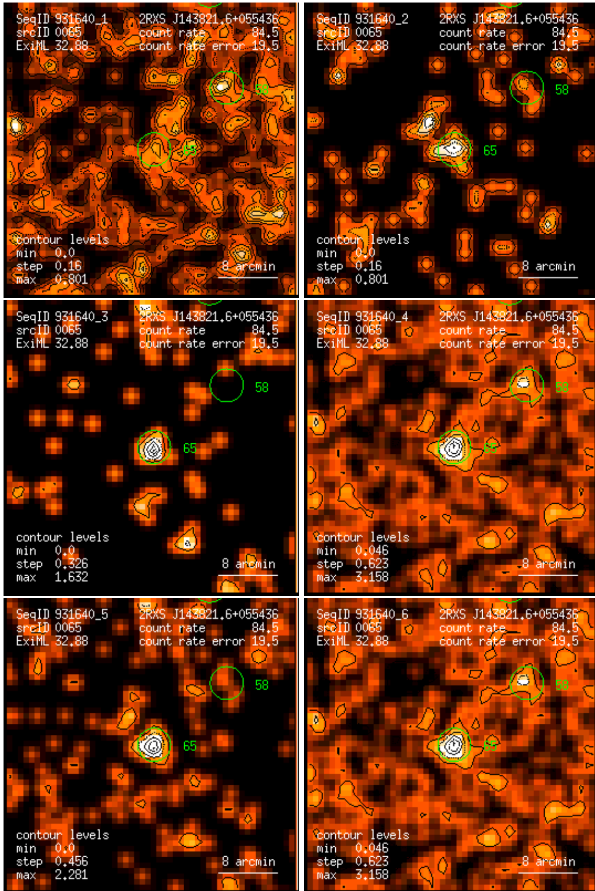
Figure 65: RASS 931640: detection 0065: band rate images, Gaussian filter: (1) PSPC channels 11 – 41, (2) 52 – 90, (3) 91 – 201, (4) 11 – 235, (5) 52 – 201, (6) 11 – 201. Broad band rates in counts/ks. Band rate contour levels in counts/ks/arcmin 2 .
