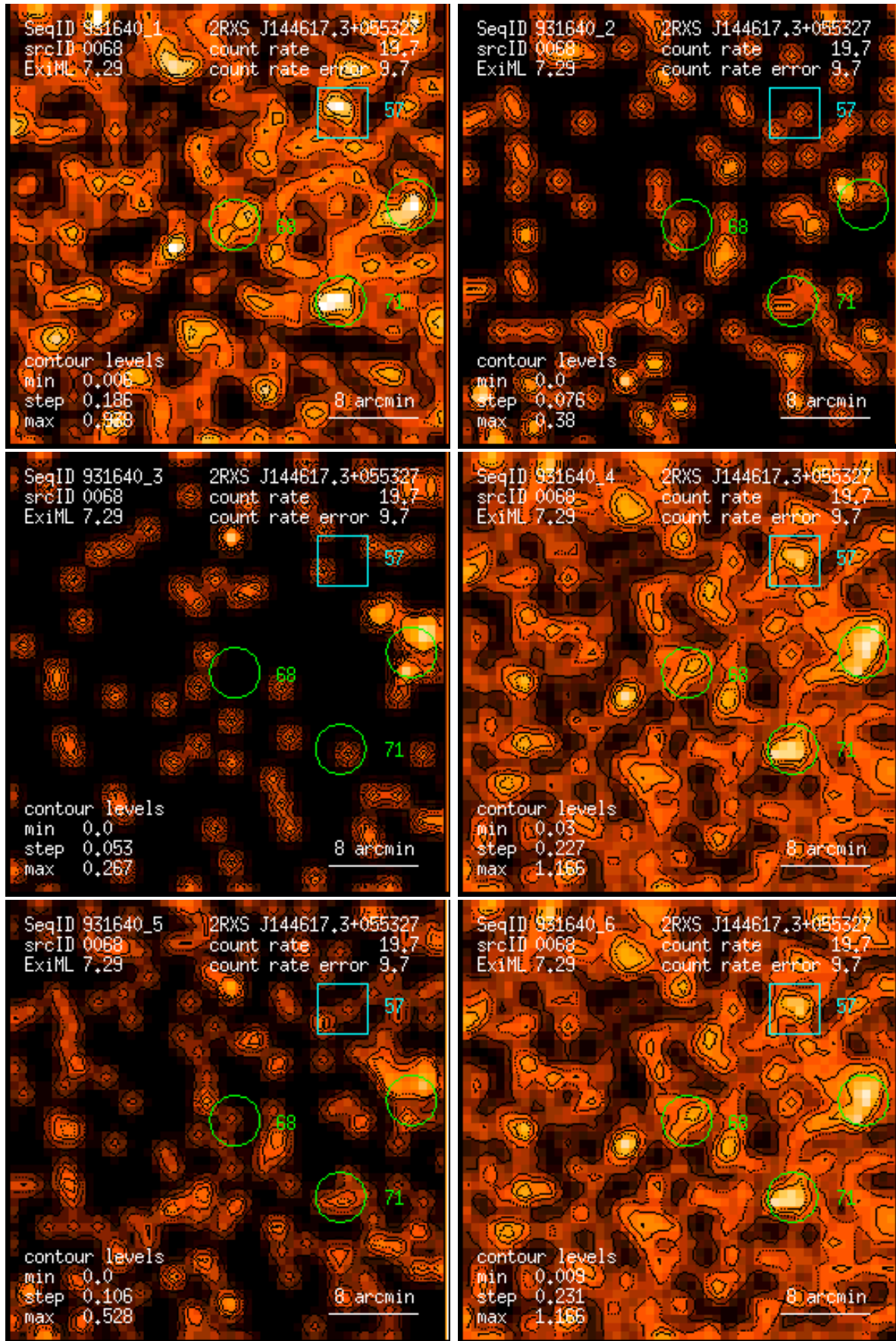
Figure 68: RASS 931640: detection 0068: band rate images, Gaussian filter: (1) PSPC channels 11 – 41, (2) 52 – 90, (3) 91 – 201, (4) 11 – 235, (5) 52 – 201, (6) 11 – 201. Broad band rates in counts/ks. Band rate contour levels in counts/ks/arcmin 2 .
