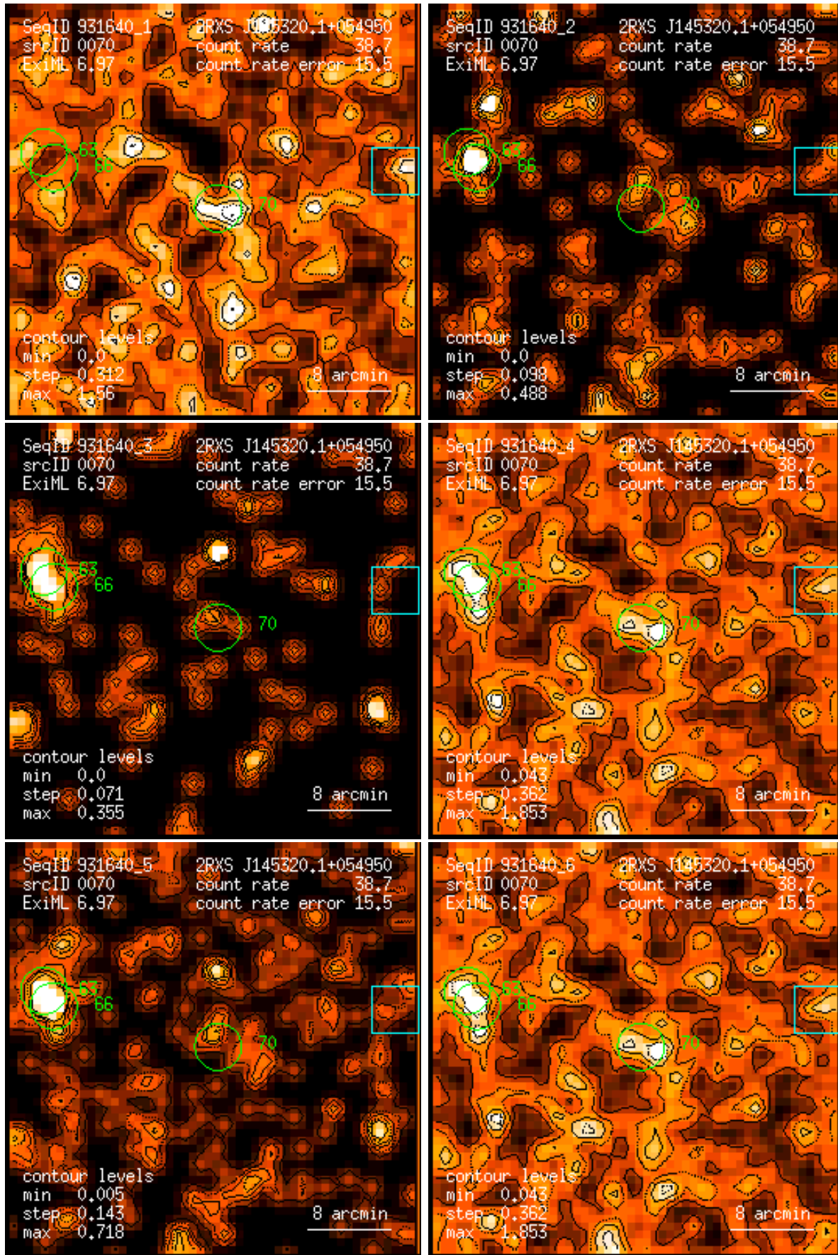
Figure 70: RASS 931640: detection 0070: band rate images, Gaussian filter: (1) PSPC channels 11 – 41, (2) 52 – 90, (3) 91 – 201, (4) 11 – 235, (5) 52 – 201, (6) 11 – 201. Broad band rates in counts/ks. Band rate contour levels in counts/ks/arcmin 2 .
