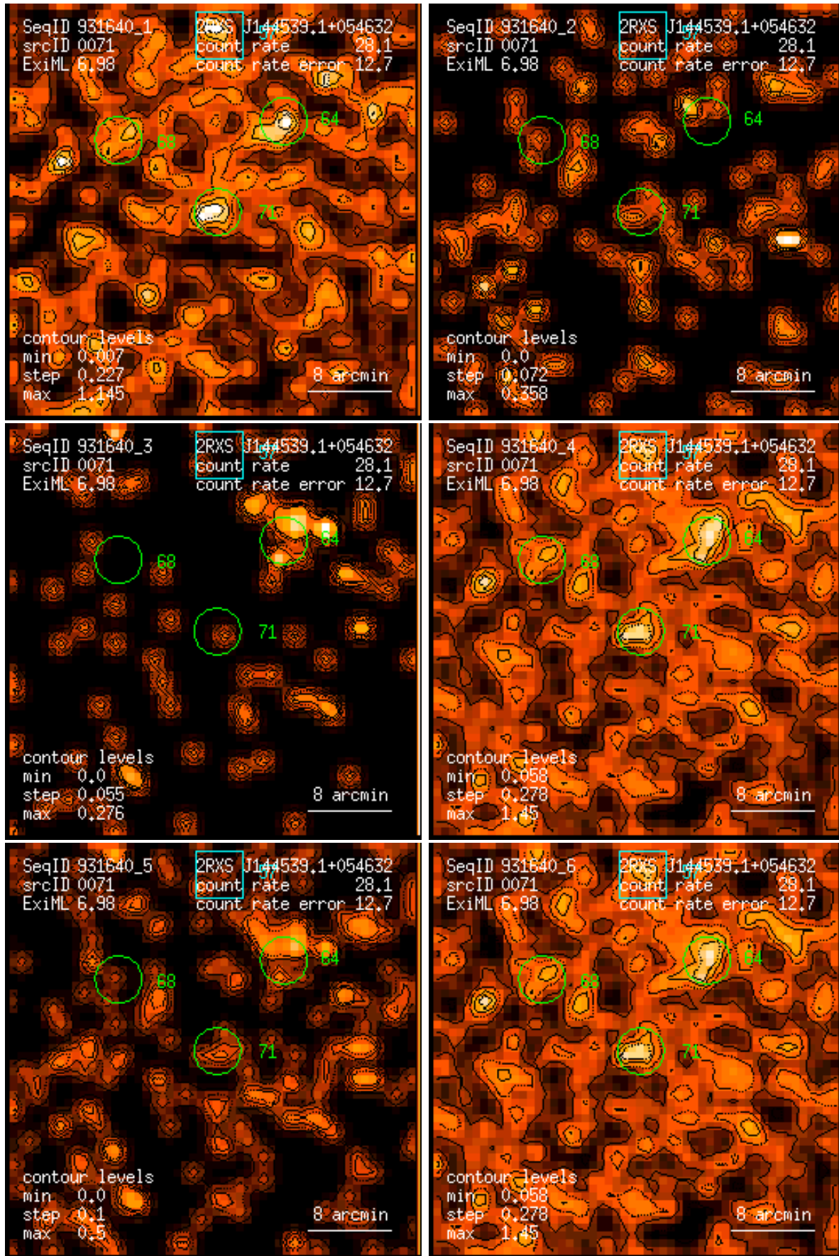
Figure 71: RASS 931640: detection 0071: band rate images, Gaussian filter: (1) PSPC channels 11 – 41, (2) 52 – 90, (3) 91 – 201, (4) 11 – 235, (5) 52 – 201, (6) 11 – 201. Broad band rates in counts/ks. Band rate contour levels in counts/ks/arcmin 2 .
