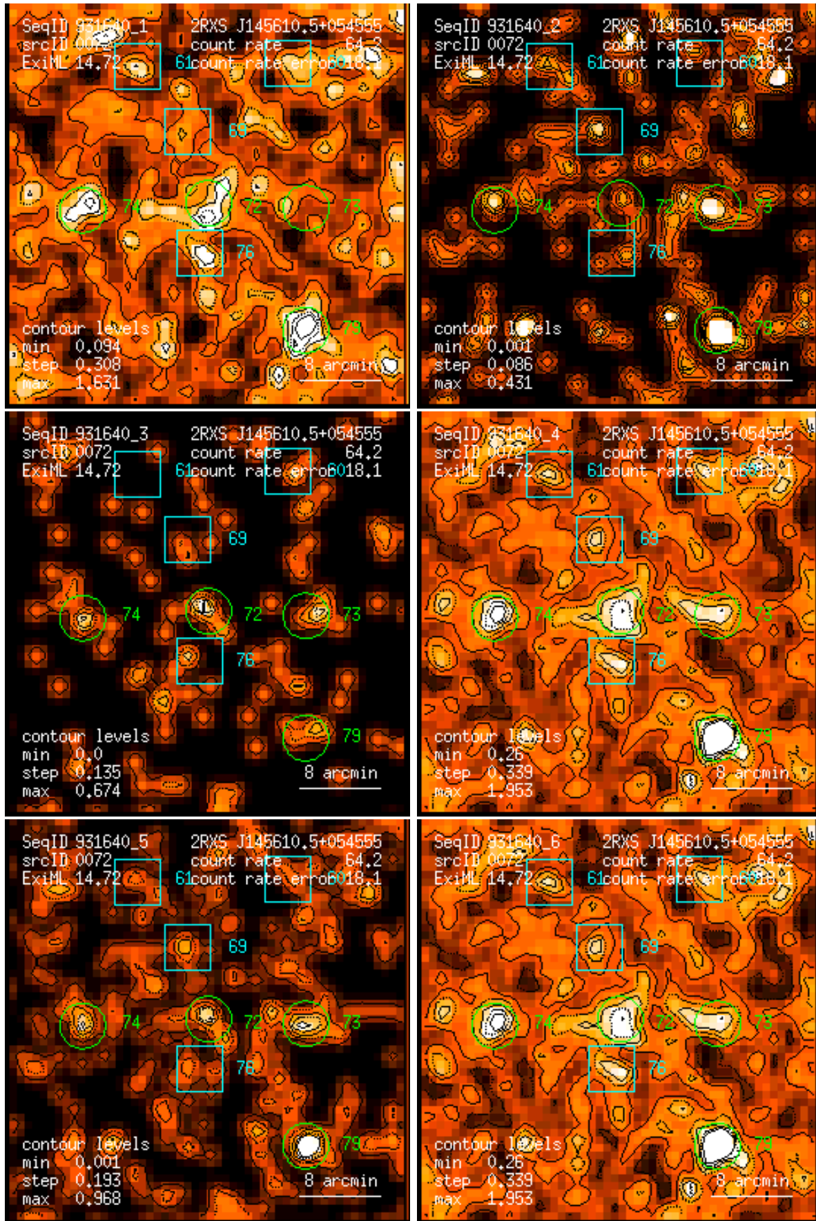
Figure 72: RASS 931640: detection 0072: band rate images, Gaussian filter: (1) PSPC channels 11 – 41, (2) 52 – 90, (3) 91 – 201, (4) 11 – 235, (5) 52 – 201, (6) 11 – 201. Broad band rates in counts/ks. Band rate contour levels in counts/ks/arcmin 2 .
