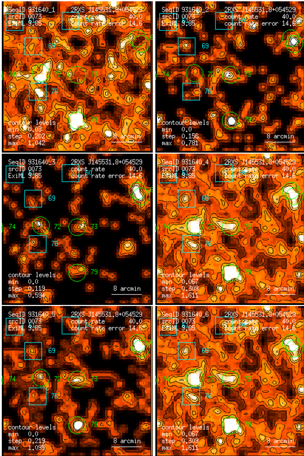
Figure 73: RASS 931640: detection 0073: band rate images, Gaussian filter: (1) PSPC channels 11 – 41, (2) 52 – 90, (3) 91 – 201, (4) 11 – 235, (5) 52 – 201, (6) 11 – 201. Broad band rates in counts/ks. Band rate contour levels in counts/ks/arcmin 2 .
