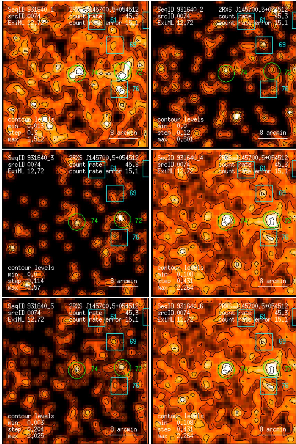
Figure 74: RASS 931640: detection 0074: band rate images, Gaussian filter: (1) PSPC channels 11 – 41, (2) 52 – 90, (3) 91 – 201, (4) 11 – 235, (5) 52 – 201, (6) 11 – 201. Broad band rates in counts/ks. Band rate contour levels in counts/ks/arcmin 2 .
