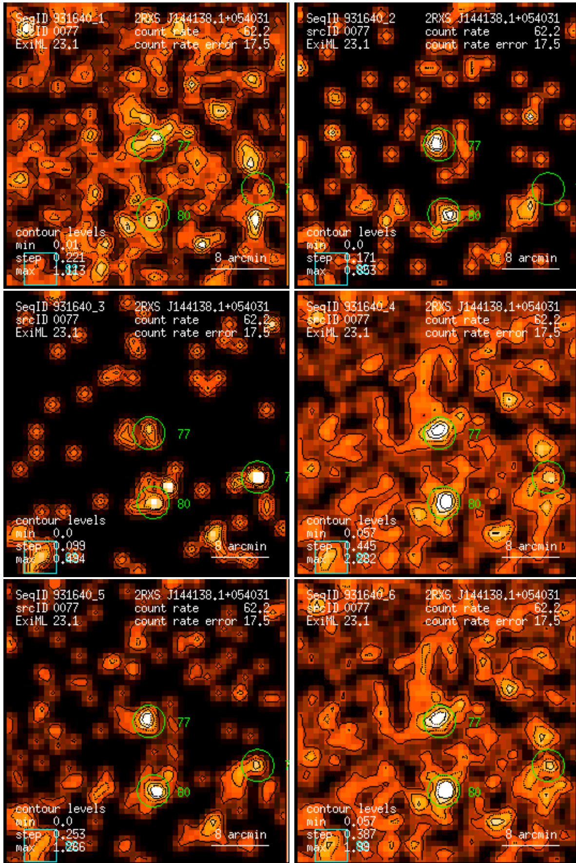
Figure 77: RASS 931640: detection 0077: band rate images, Gaussian filter: (1) PSPC channels 11 – 41, (2) 52 – 90, (3) 91 – 201, (4) 11 – 235, (5) 52 – 201, (6) 11 – 201. Broad band rates in counts/ks. Band rate contour levels in counts/ks/arcmin 2 .
