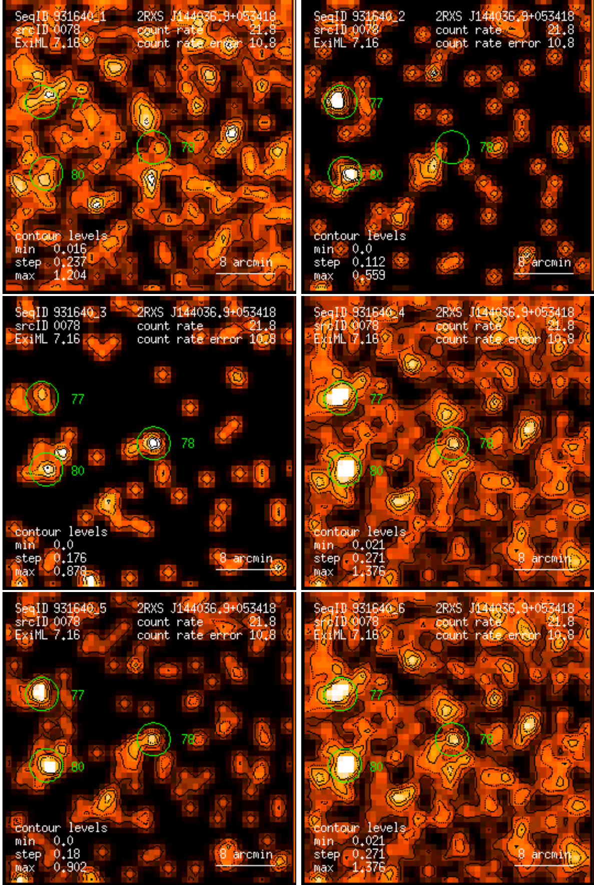
Figure 78: RASS 931640: detection 0078: band rate images, Gaussian filter: (1) PSPC channels 11 – 41, (2) 52 – 90, (3) 91 – 201, (4) 11 – 235, (5) 52 – 201, (6) 11 – 201. Broad band rates in counts/ks. Band rate contour levels in counts/ks/arcmin 2 .
