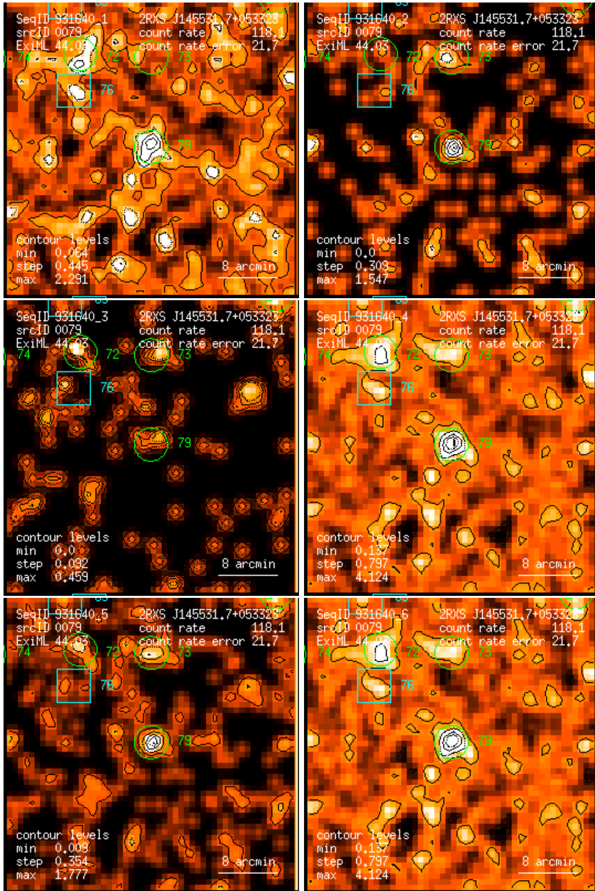
Figure 79: RASS 931640: detection 0079: band rate images, Gaussian filter: (1) PSPC channels 11 – 41, (2) 52 – 90, (3) 91 – 201, (4) 11 – 235, (5) 52 – 201, (6) 11 – 201. Broad band rates in counts/ks. Band rate contour levels in counts/ks/arcmin 2 .
