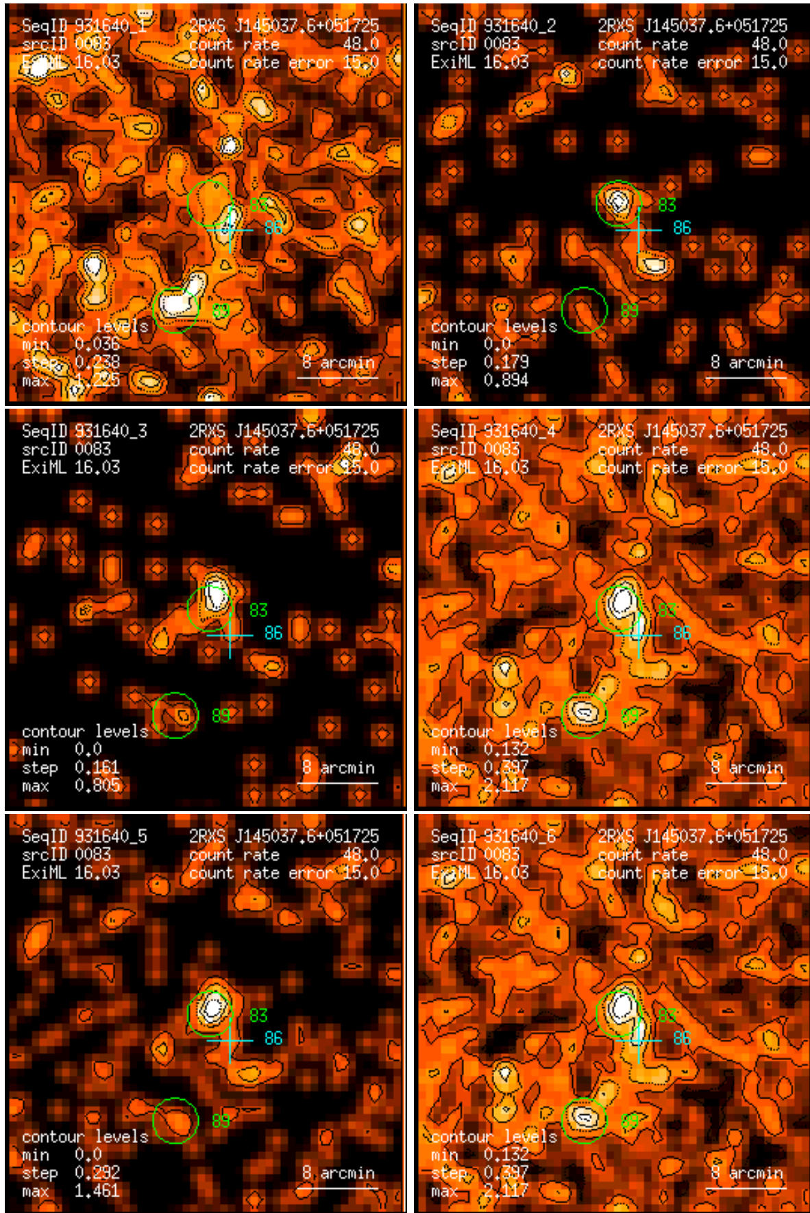
Figure 83: RASS 931640: detection 0083: band rate images, Gaussian filter: (1) PSPC channels 11 – 41, (2) 52 – 90, (3) 91 – 201, (4) 11 – 235, (5) 52 – 201, (6) 11 – 201. Broad band rates in counts/ks. Band rate contour levels in counts/ks/arcmin 2 .
