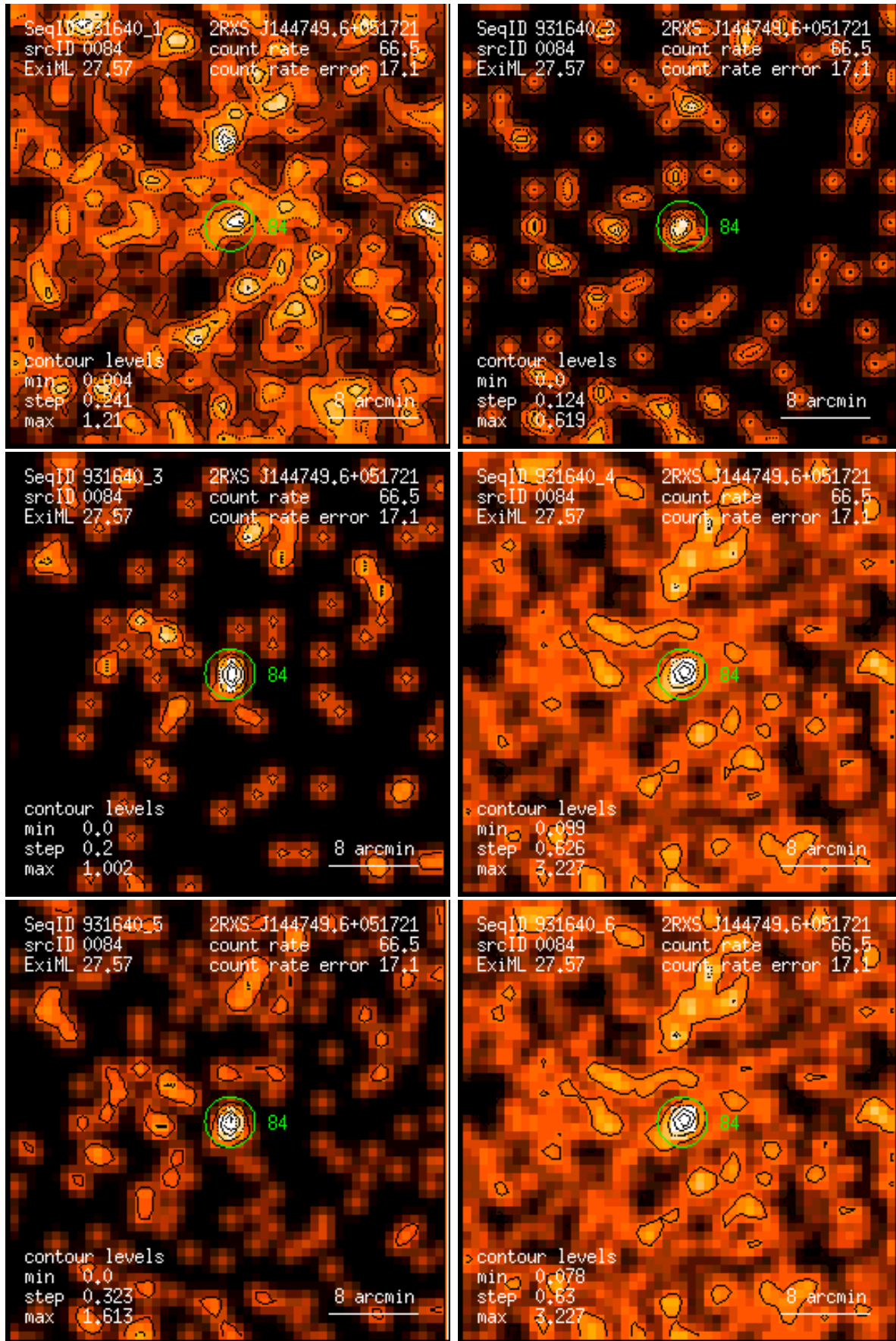
Figure 84: RASS 931640: detection 0084: band rate images, Gaussian filter: (1) PSPC channels 11 – 41, (2) 52 – 90, (3) 91 – 201, (4) 11 – 235, (5) 52 – 201, (6) 11 – 201. Broad band rates in counts/ks. Band rate contour levels in counts/ks/arcmin 2 .
