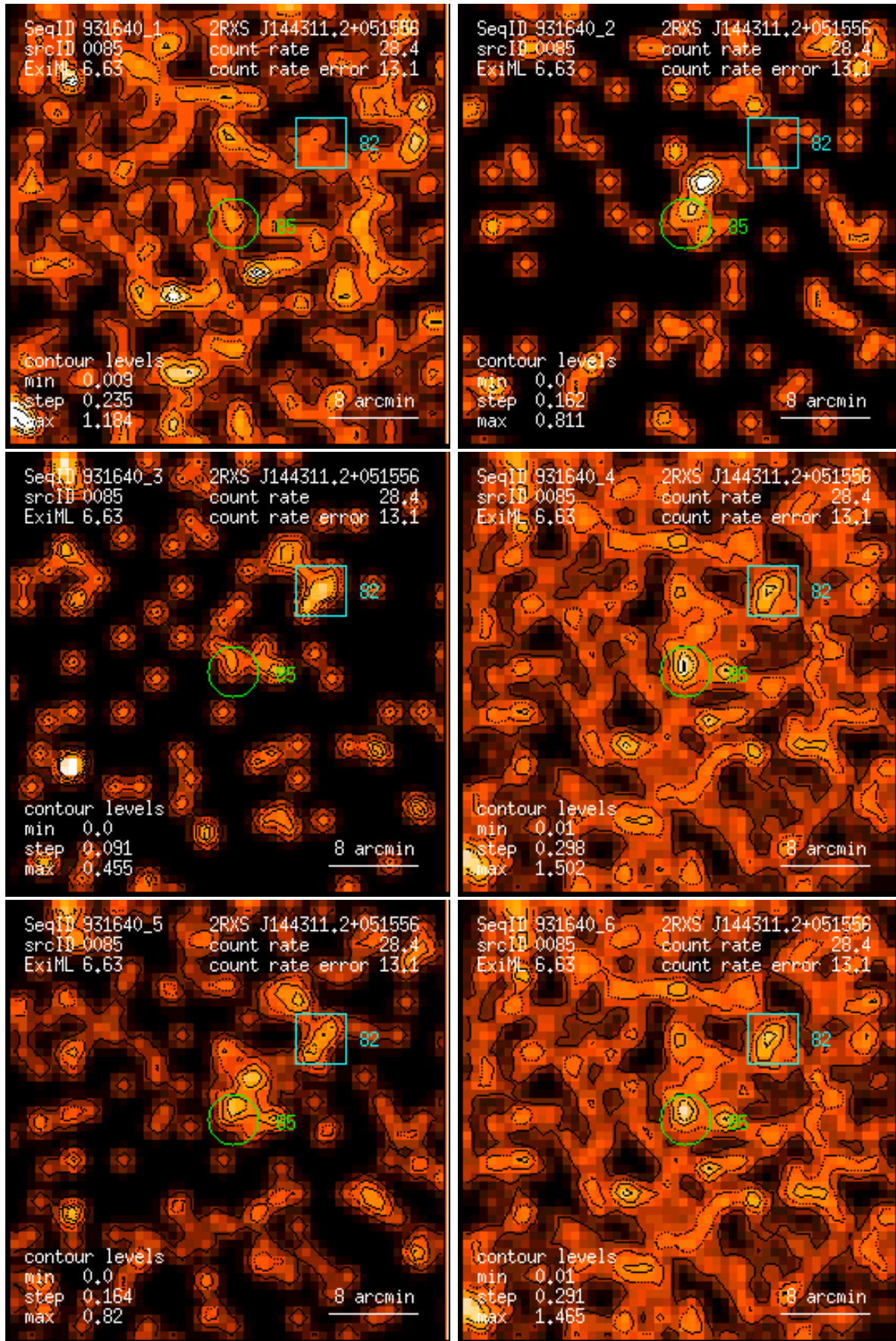
Figure 85: RASS 931640: detection 0085: band rate images, Gaussian filter: (1) PSPC channels 11 – 41, (2) 52 – 90, (3) 91 – 201, (4) 11 – 235, (5) 52 – 201, (6) 11 – 201. Broad band rates in counts/ks. Band rate contour levels in counts/ks/arcmin 2 .
