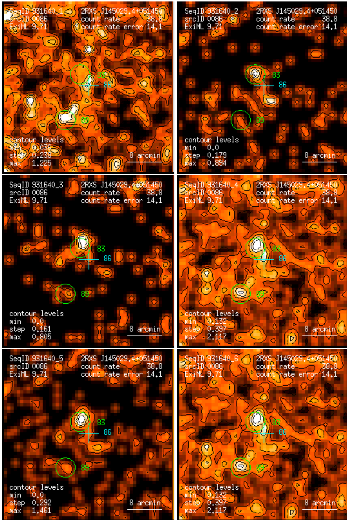
Figure 86: RASS 931640: detection 0086: band rate images, Gaussian filter: (1) PSPC channels 11 – 41, (2) 52 – 90, (3) 91 – 201, (4) 11 – 235, (5) 52 – 201, (6) 11 – 201. Broad band rates in counts/ks. Band rate contour levels in counts/ks/arcmin 2 .
