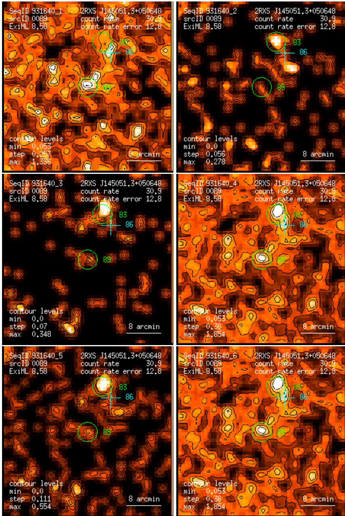
Figure 89: RASS 931640: detection 0089: band rate images, Gaussian filter: (1) PSPC channels 11 – 41, (2) 52 – 90, (3) 91 – 201, (4) 11 – 235, (5) 52 – 201, (6) 11 – 201. Broad band rates in counts/ks. Band rate contour levels in counts/ks/arcmin 2 .
