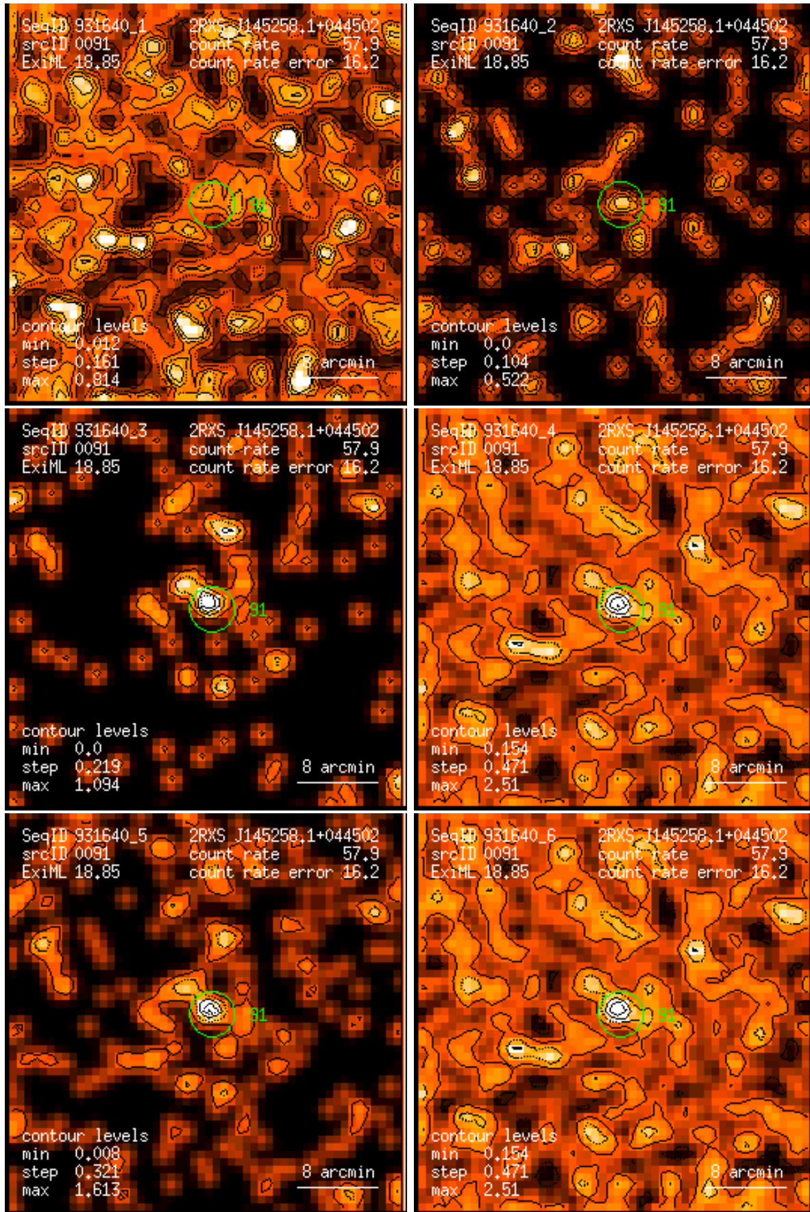
Figure 91: RASS 931640: detection 0091: band rate images, Gaussian filter: (1) PSPC channels 11 – 41, (2) 52 – 90, (3) 91 – 201, (4) 11 – 235, (5) 52 – 201, (6) 11 – 201. Broad band rates in counts/ks. Band rate contour levels in counts/ks/arcmin 2 .
