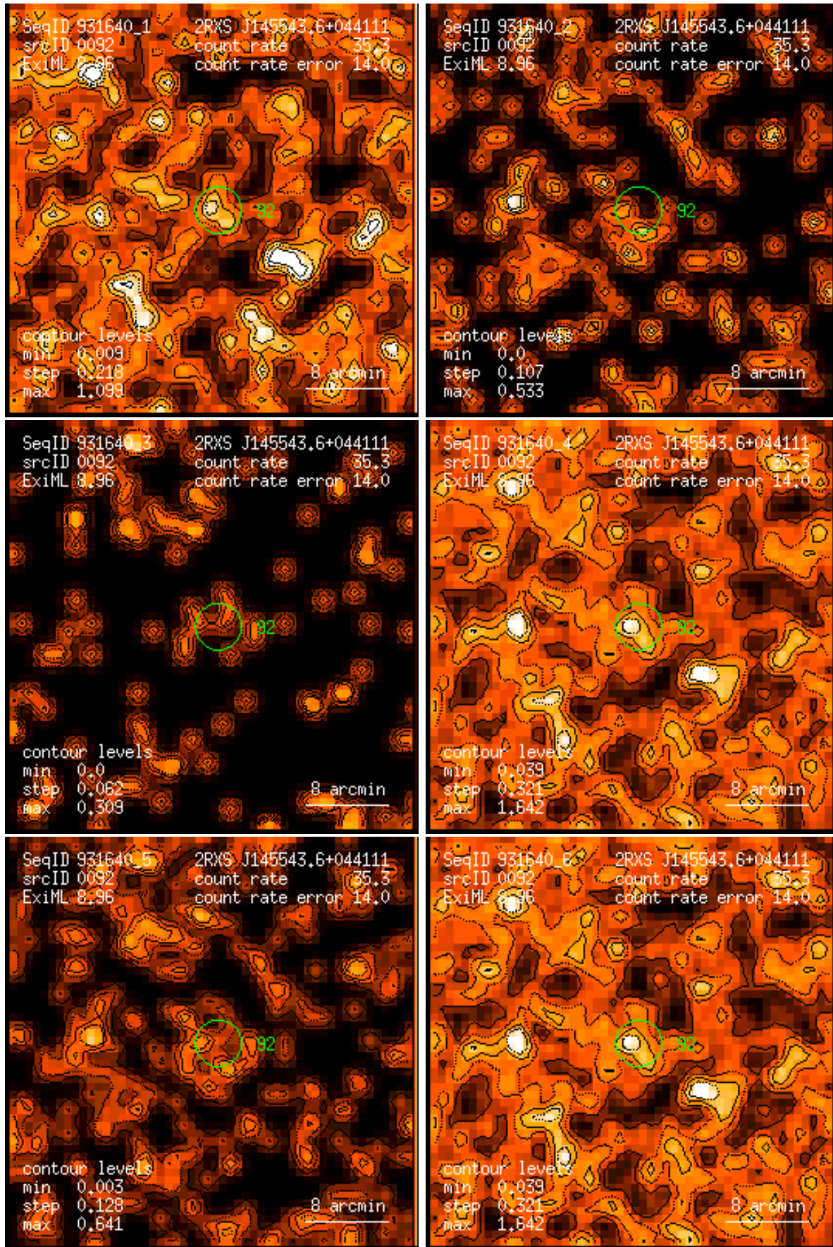
Figure 92: RASS 931640: detection 0092: band rate images, Gaussian filter: (1) PSPC channels 11 – 41, (2) 52 – 90, (3) 91 – 201, (4) 11 – 235, (5) 52 – 201, (6) 11 – 201. Broad band rates in counts/ks. Band rate contour levels in counts/ks/arcmin 2 .
